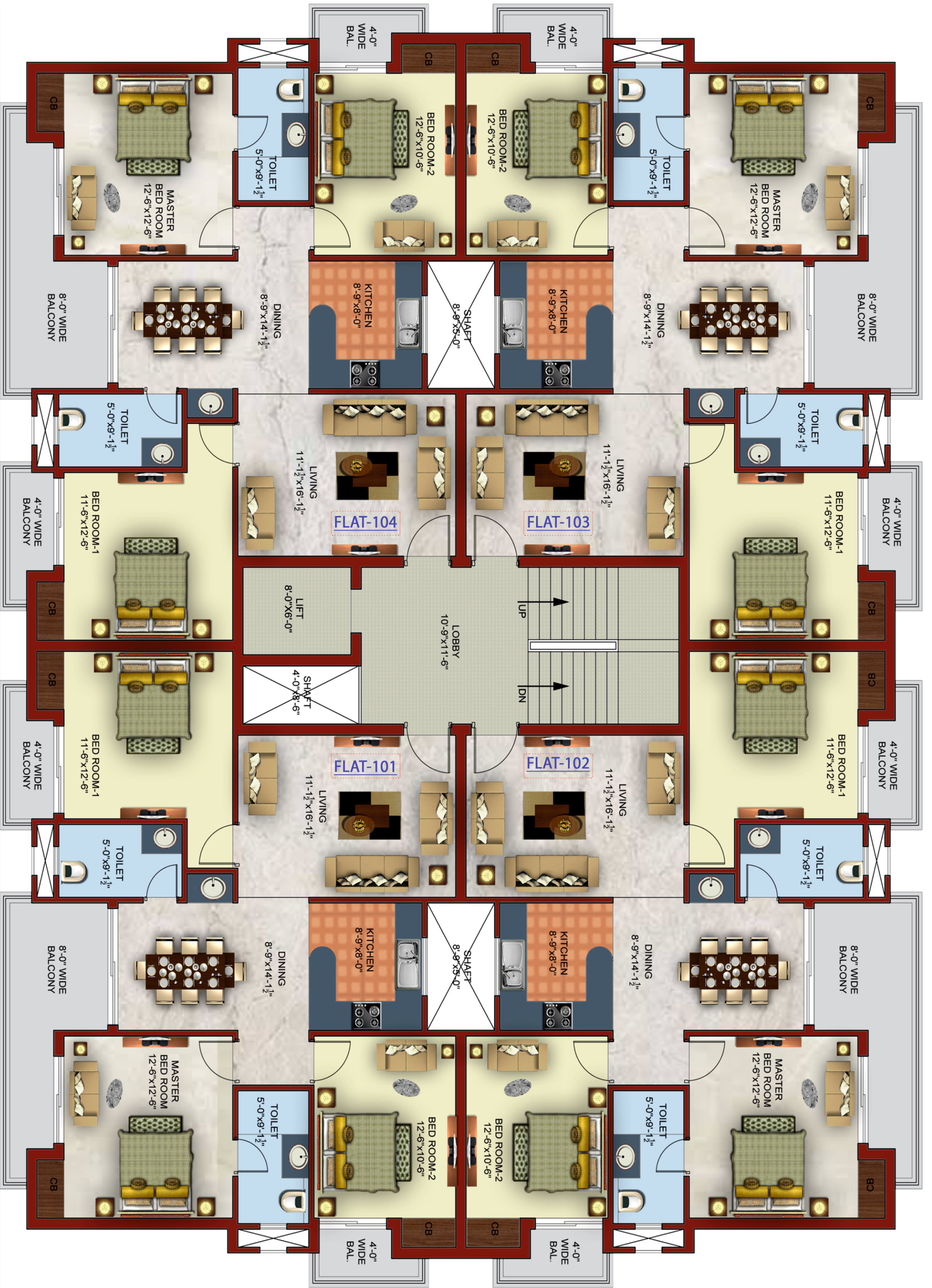
TYPICAL FLOOR PLAN (FIRST FLOOR TO FOURTH FLOOR)
