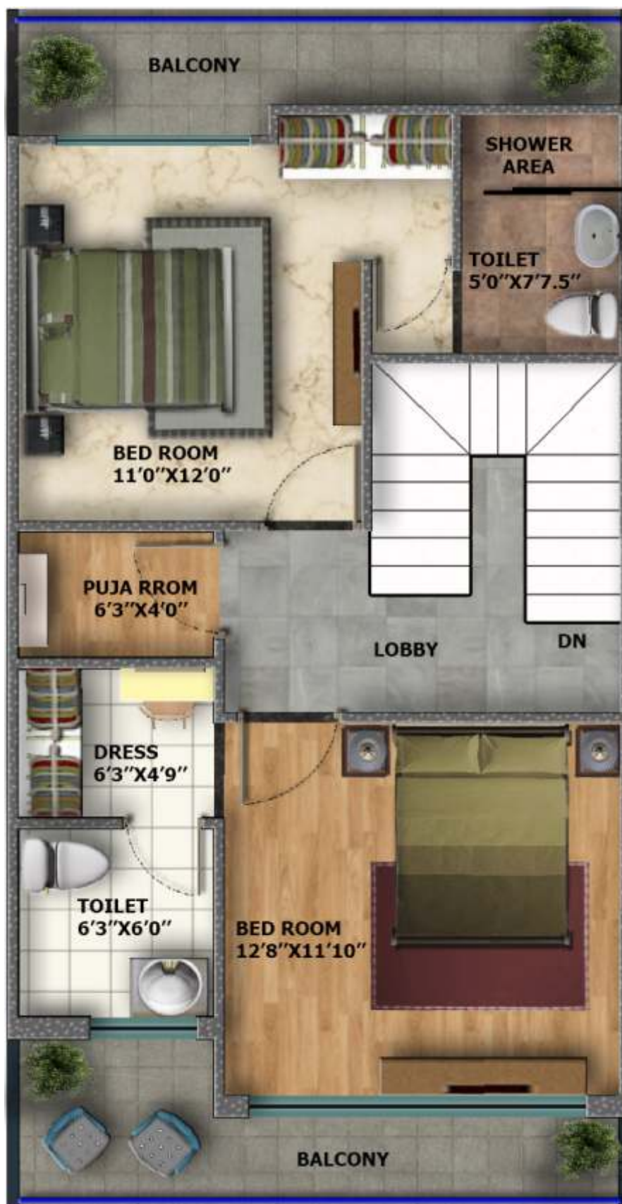
3 BHK FIRST FLOOR PLAN SIZE 20'0"X45'0"
