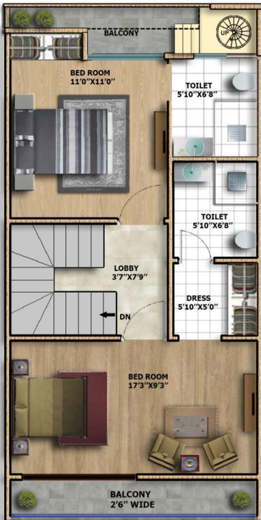
3 BHK FIRST FLOOR PLAN SIZE 18'0''X40'0''
