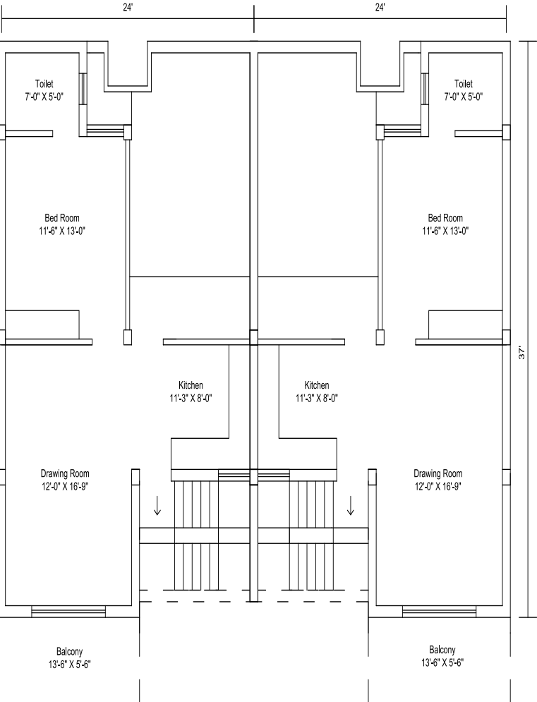
1ST FLOOR COVERED AREA 790 SFT
