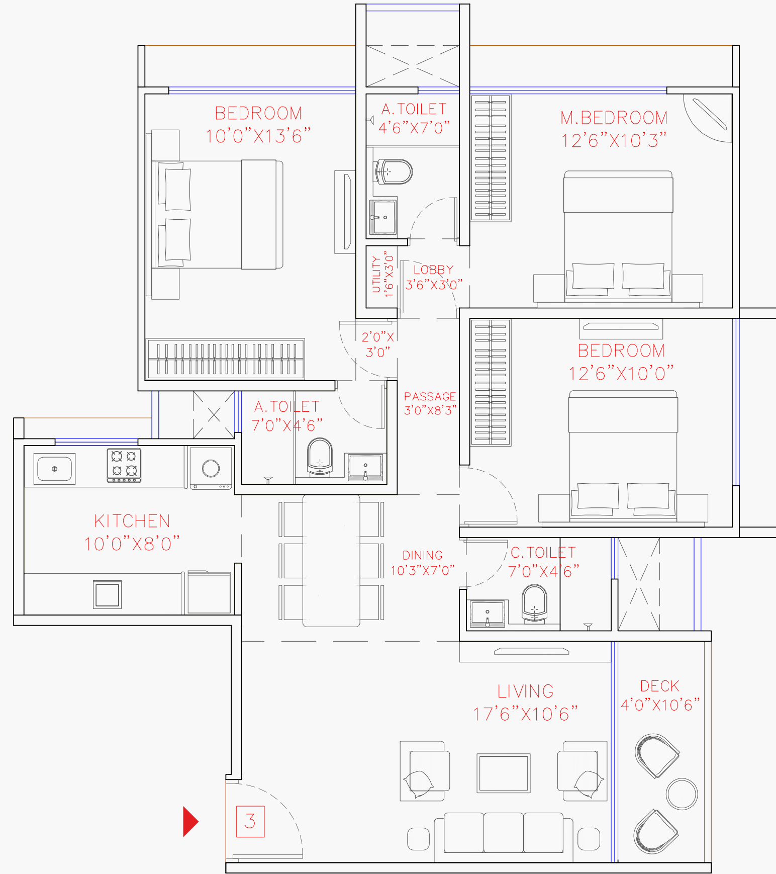
B Wing: RERA Carpet Area 953 sq. ft. Sale plan
