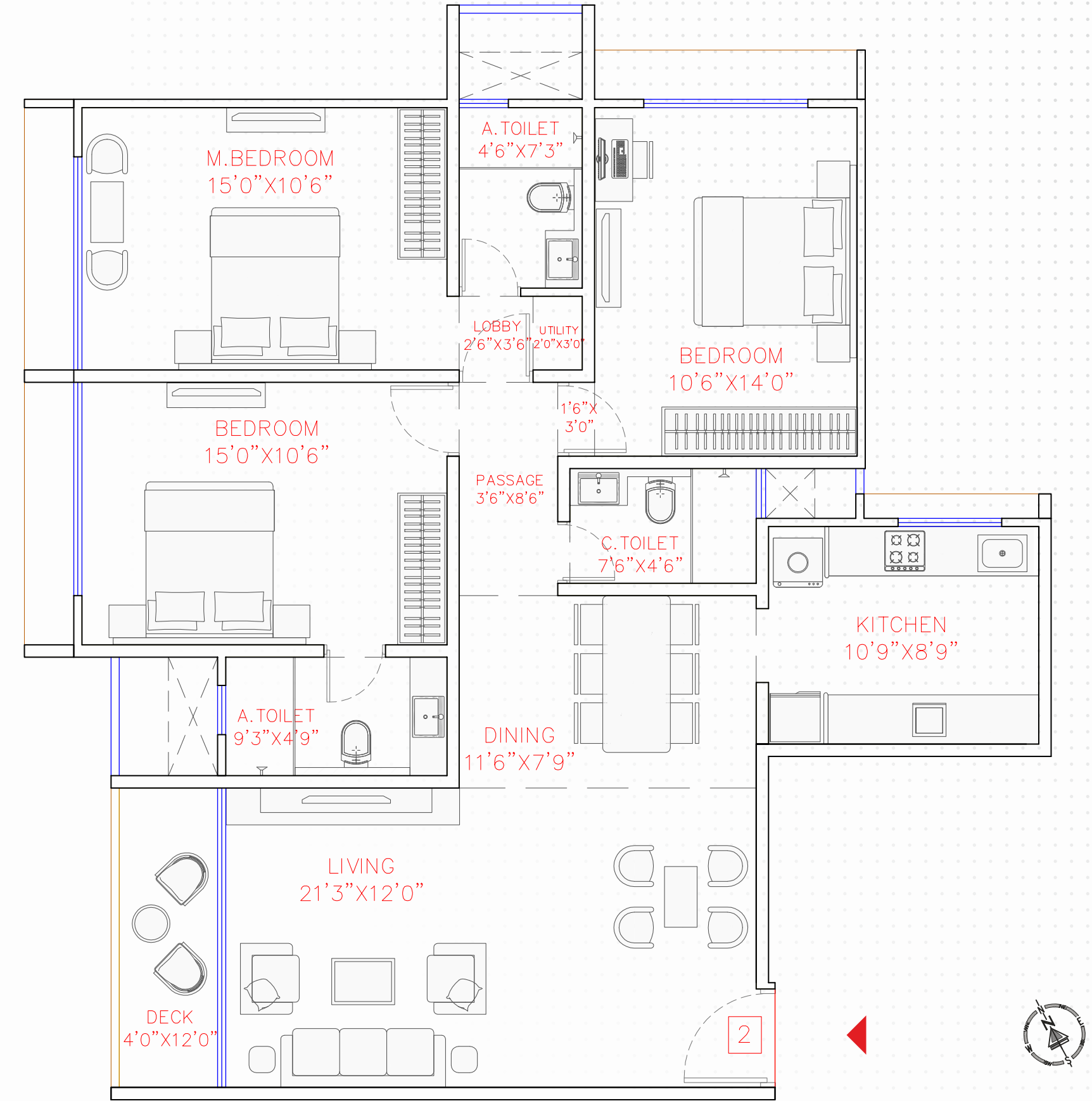
B Wing: RERA Carpet Area 1164 sq. ft. Sale plan
