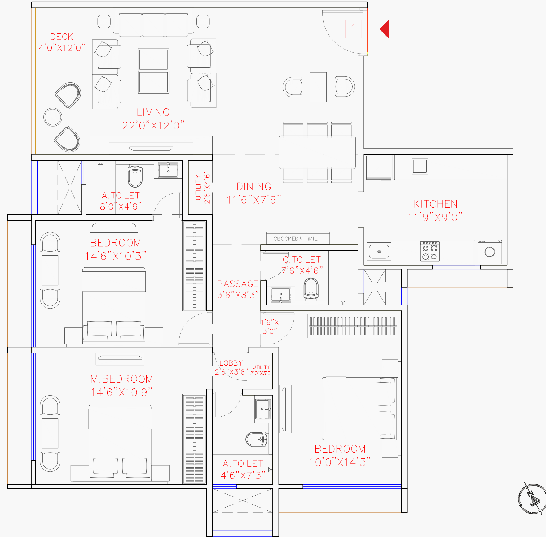
A Wing: RERA Carpet Area 1166 sq. ft. Sale plan
