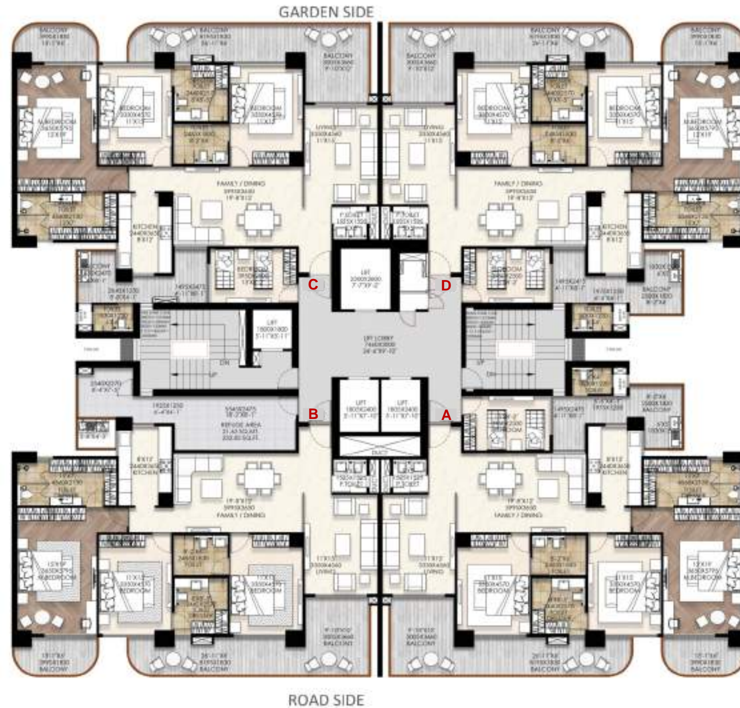
REFUGE FLOOR LEVEL 17,26 & 35 FLOOR
