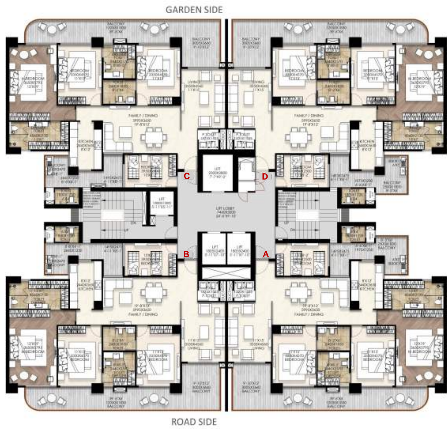
TYPICAL FLOOR LEVEL TYPICAL 4,7,10,13,16,19,22,25,28,31 & 34 FLOOR
