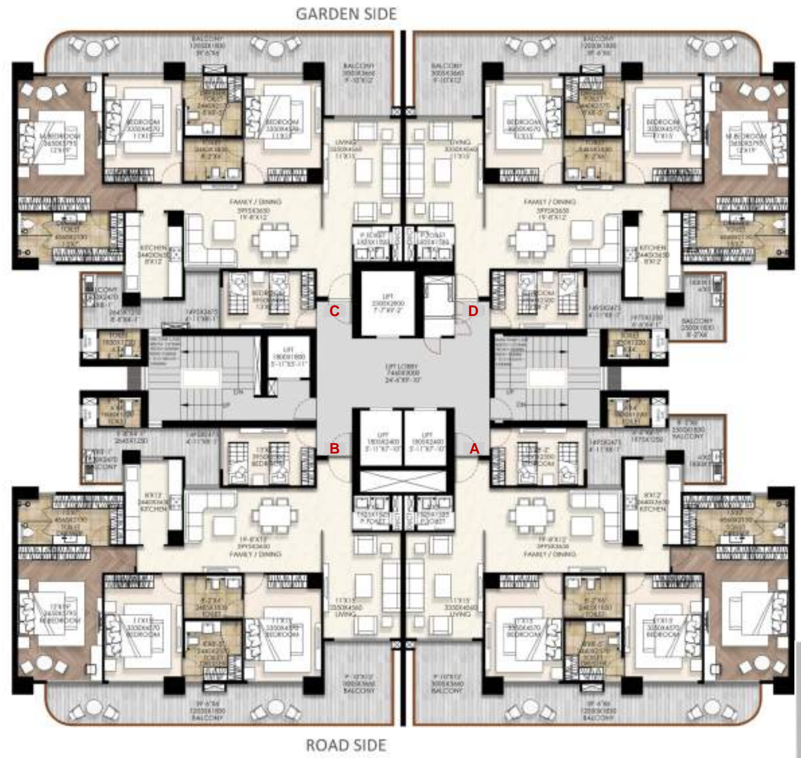
TYPICAL FLOOR LEVEL TYPICAL 1ST FLOOR
