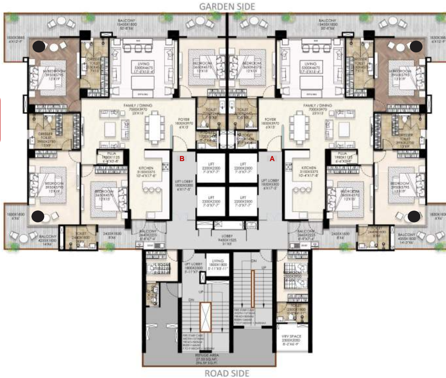
REFUGE FLOOR LEVEL TYPICAL 15,23 & 31 FLOOR
