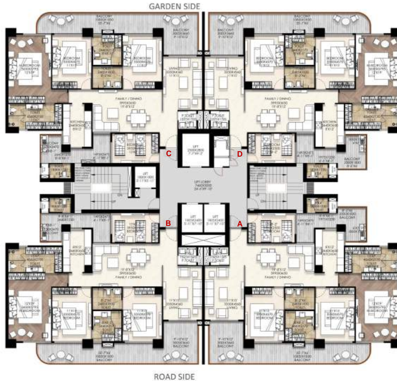
ODD FLOOR LEVEL TYPICAL 3,6,9,12,15,18,21,24,27,30,33 & 36 FLOOR
