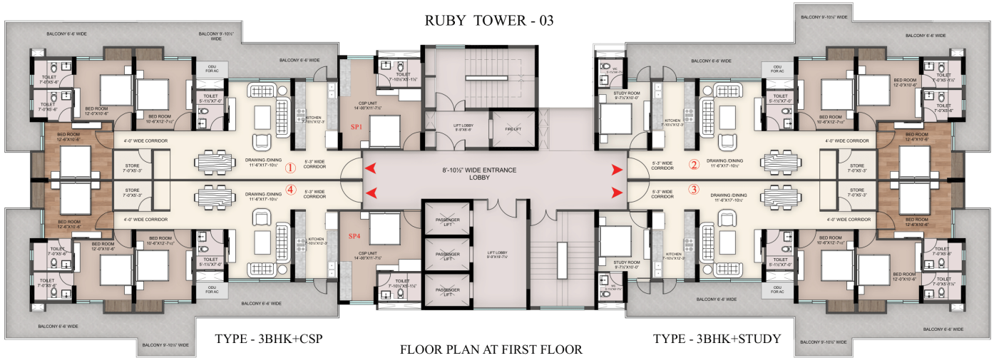
FLOOR PLAN AT FIRST FLOOR
