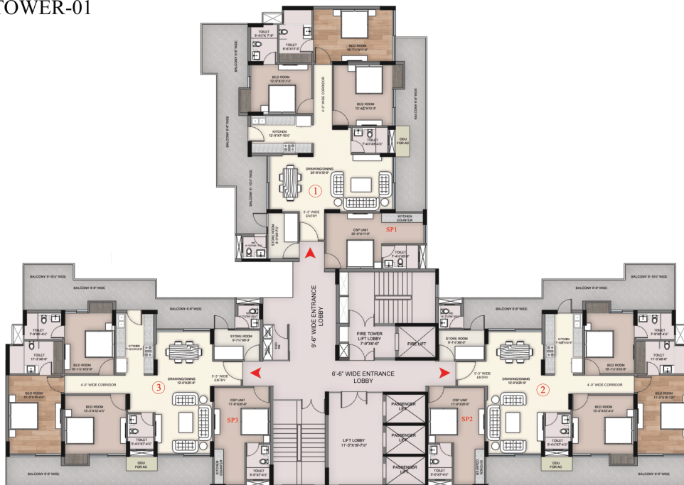
3BHK + CSP UNIT @ GROUND/ PODIUM LVL.
