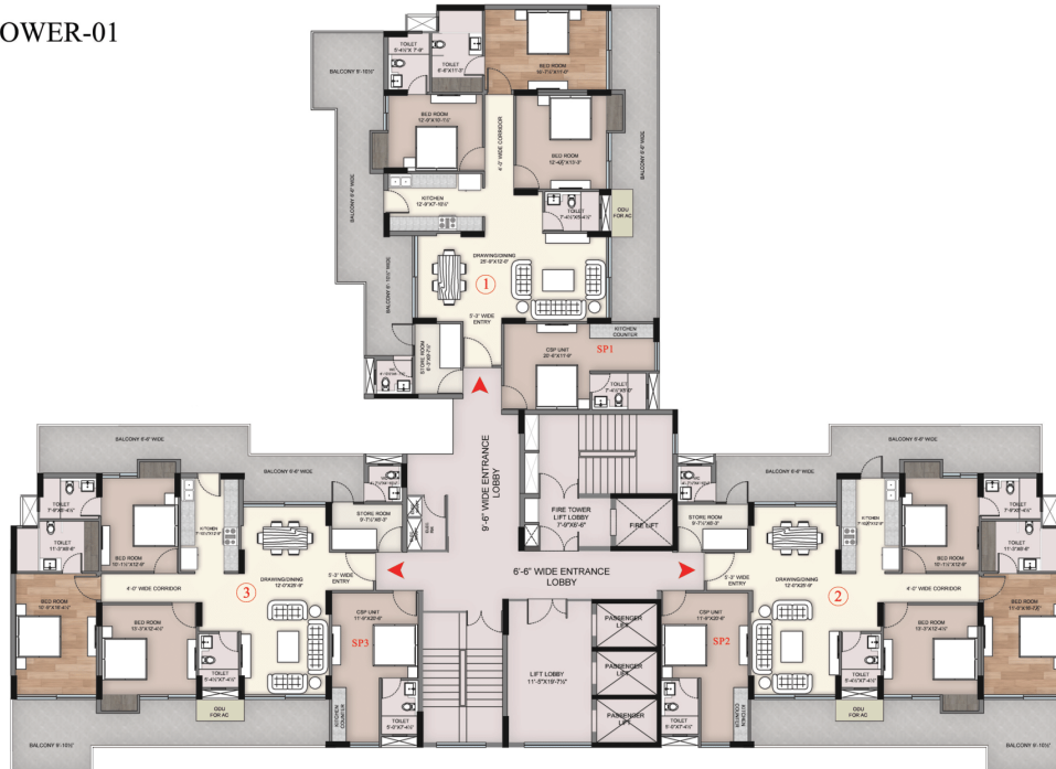
TYPE - 3BHK + CSP FLOOR PLAN AT - 3,5,7,9,11,13,15,17,19,21,23
