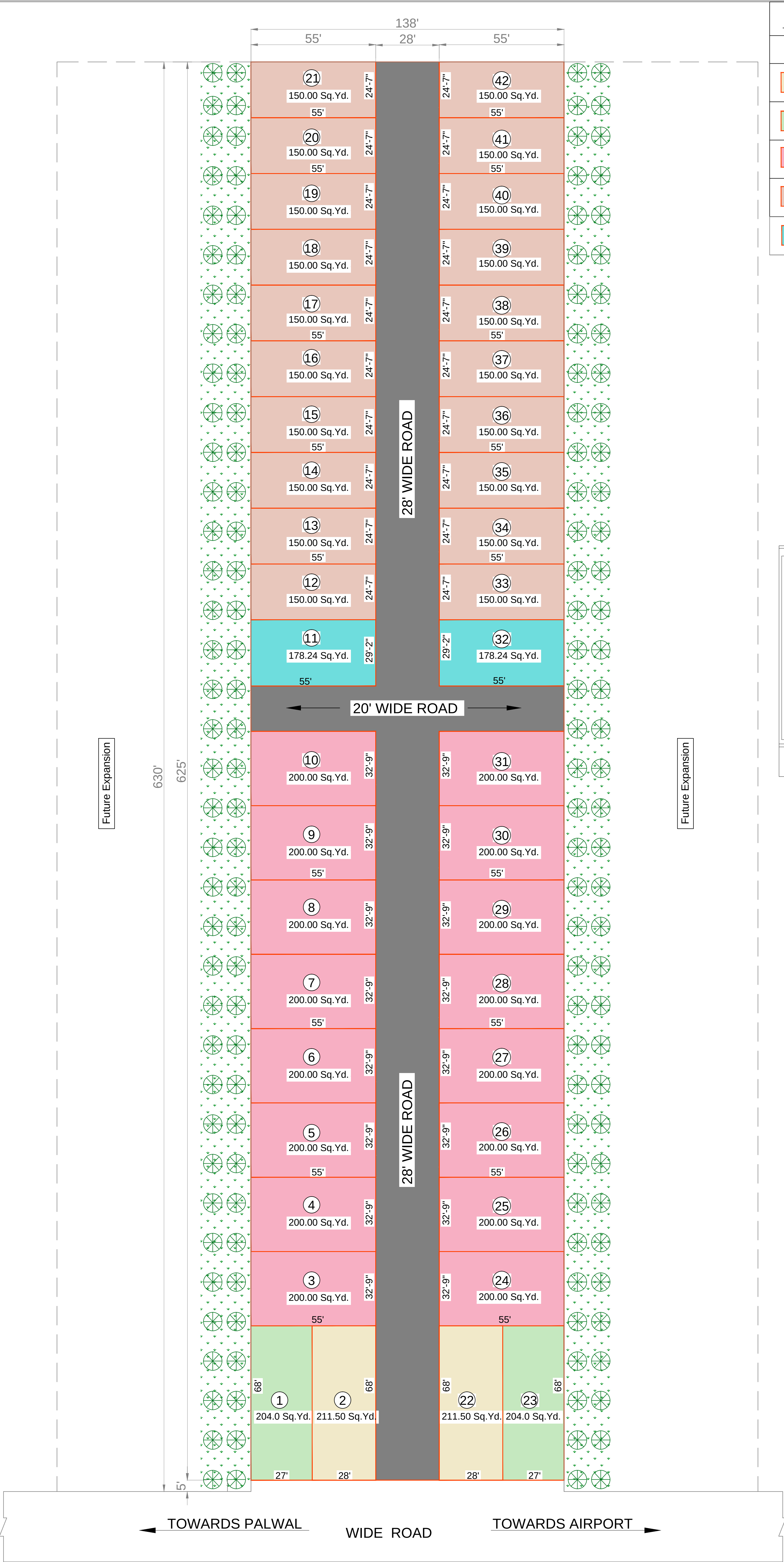
LAYOUT PLAN
