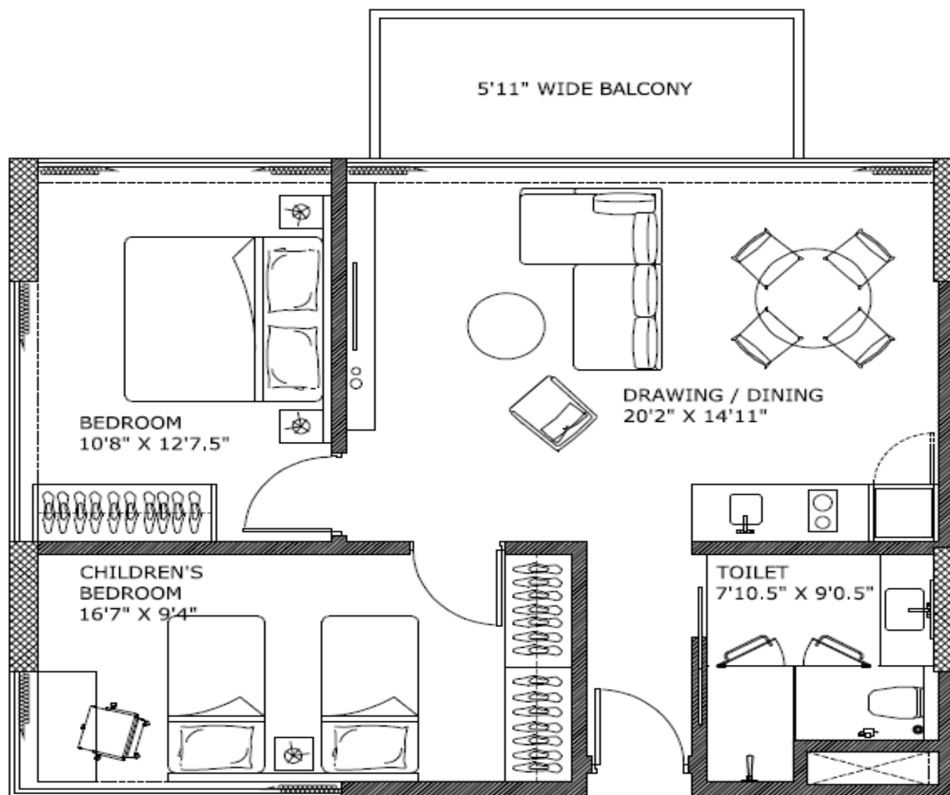
TYPICAL LAYOUT OF TYPE B (2 BED OPTION)
