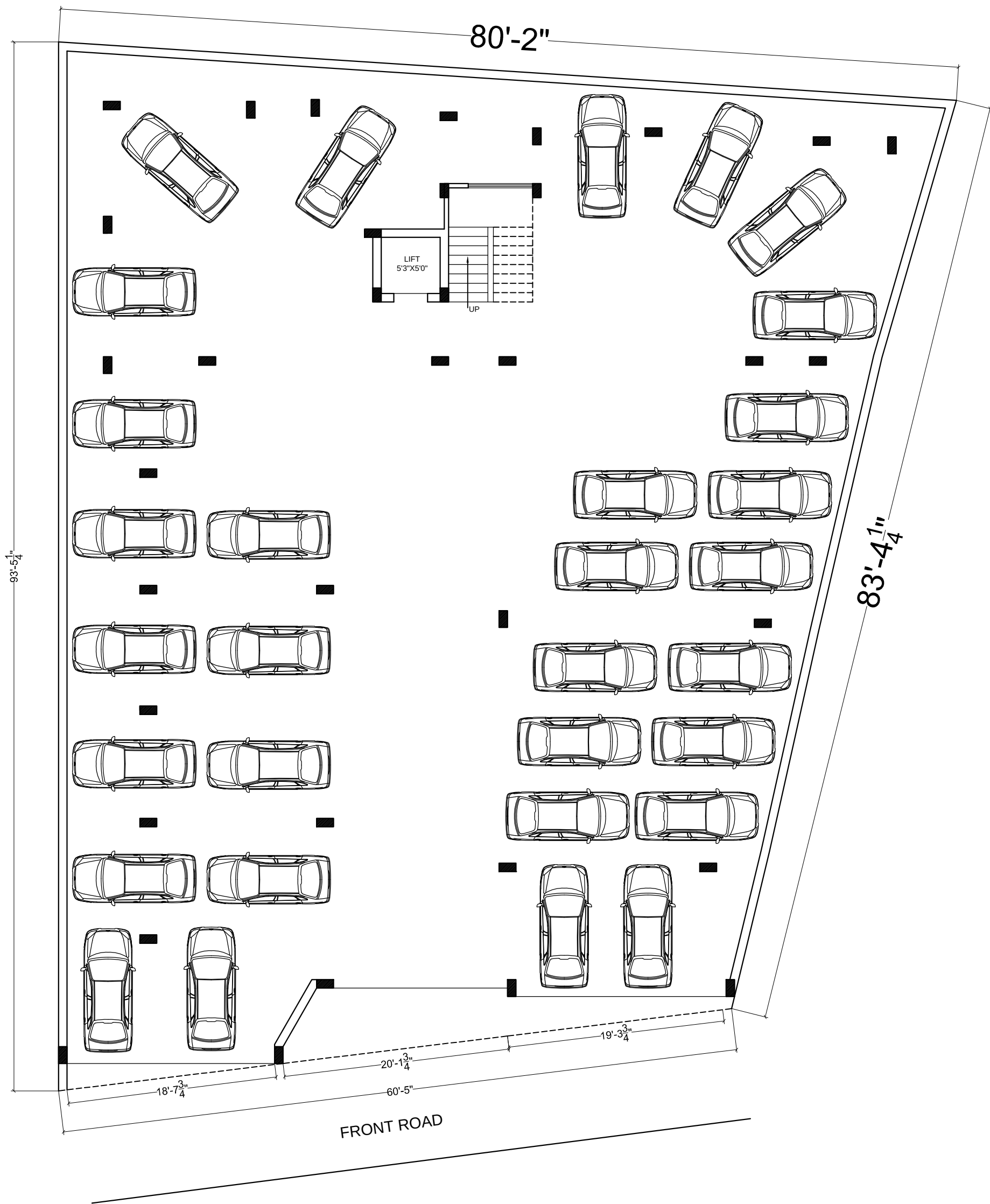
STILT FLOOR PLAN
