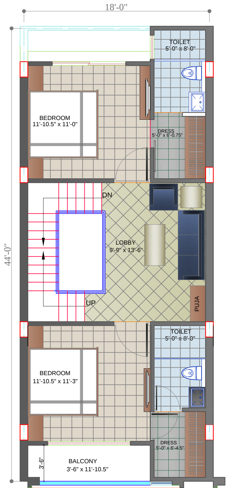
FIRST FLOOR PLAN BUILT UP AREA : 774.00 SQFT CARPET AREA : 711.03 SQFT
