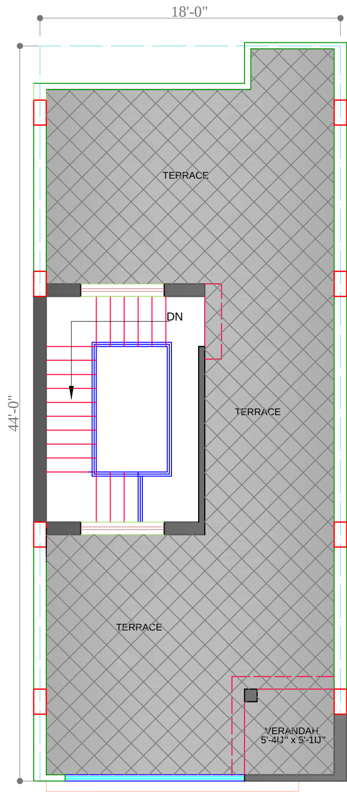
TERRACE FLOOR PLAN BUILT UP AREA : 189.00 SQFT CARPET AREA : 57.36 SQFT
