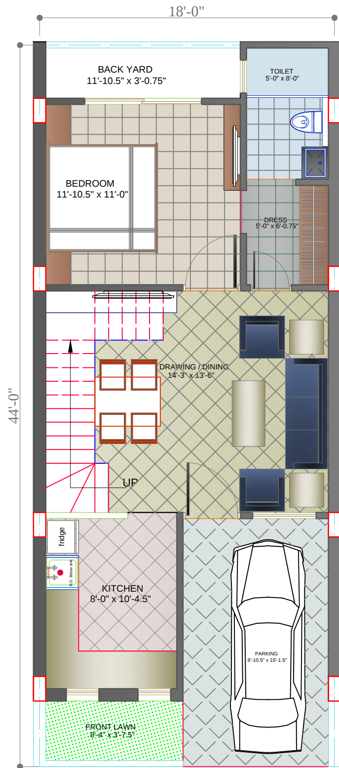
GROUND FLOOR PLAN BUILT UP AREA : 761.71 SQFT CARPET AREA : 542.15 SQFT
