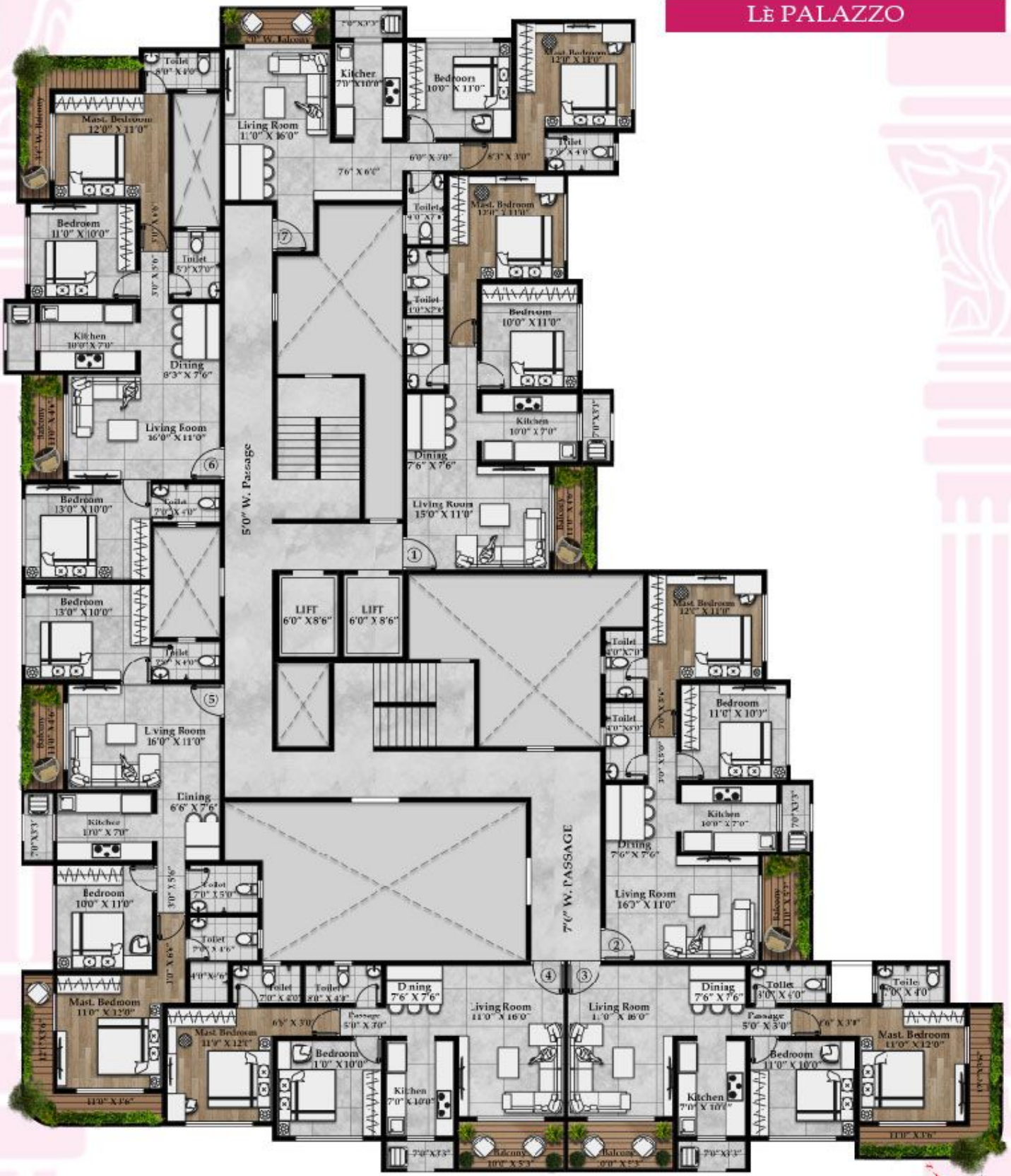
TYPICAL FLOOR ( 4 th to 6 th )
