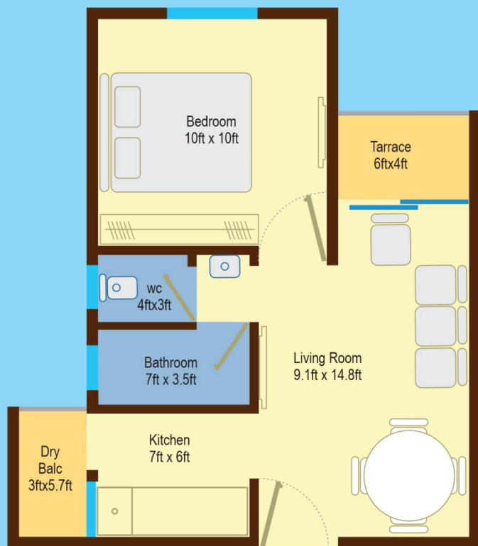
Green Valley Bldg . No.1- Sales Plan -
