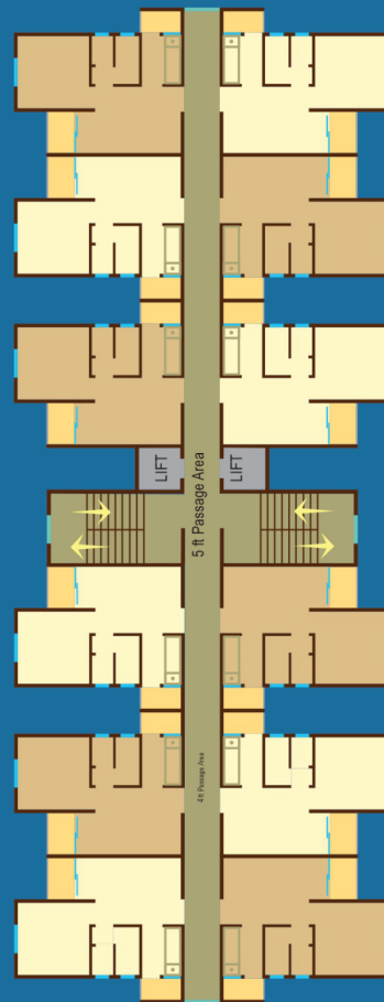
Typical Floor Plan - 1st to 10th Floor Building No. - 1.
