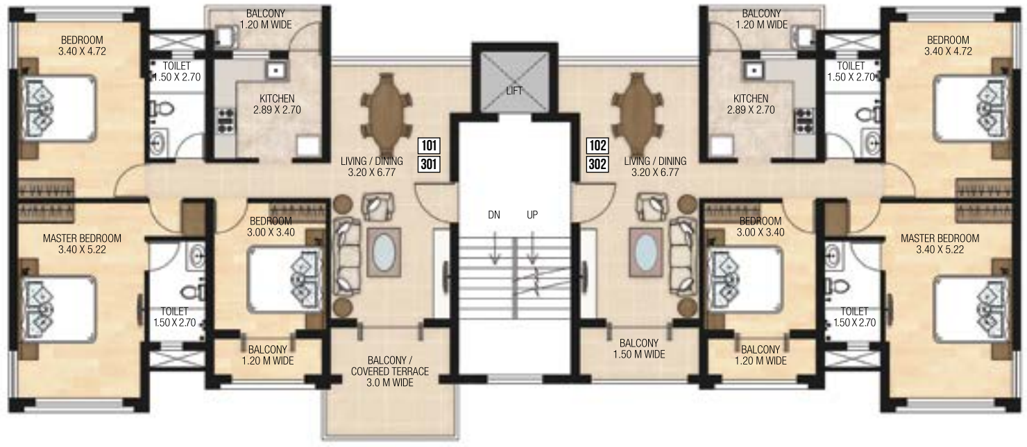
TYPICAL FIRST & THIRD FLOOR PLAN
