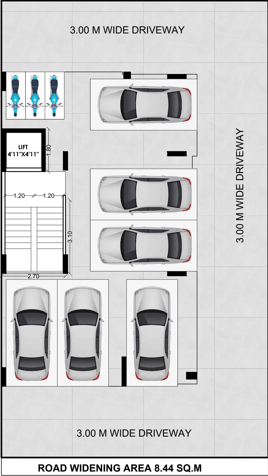
PROPOSED 9.00 M WIDE ROAD GROUND FLOOR PLAN
