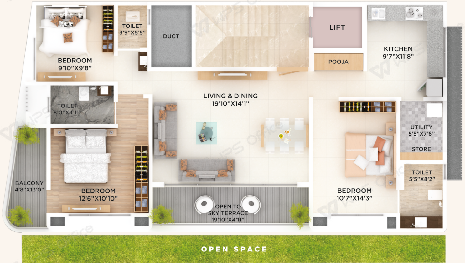
FLOOR PLAN
