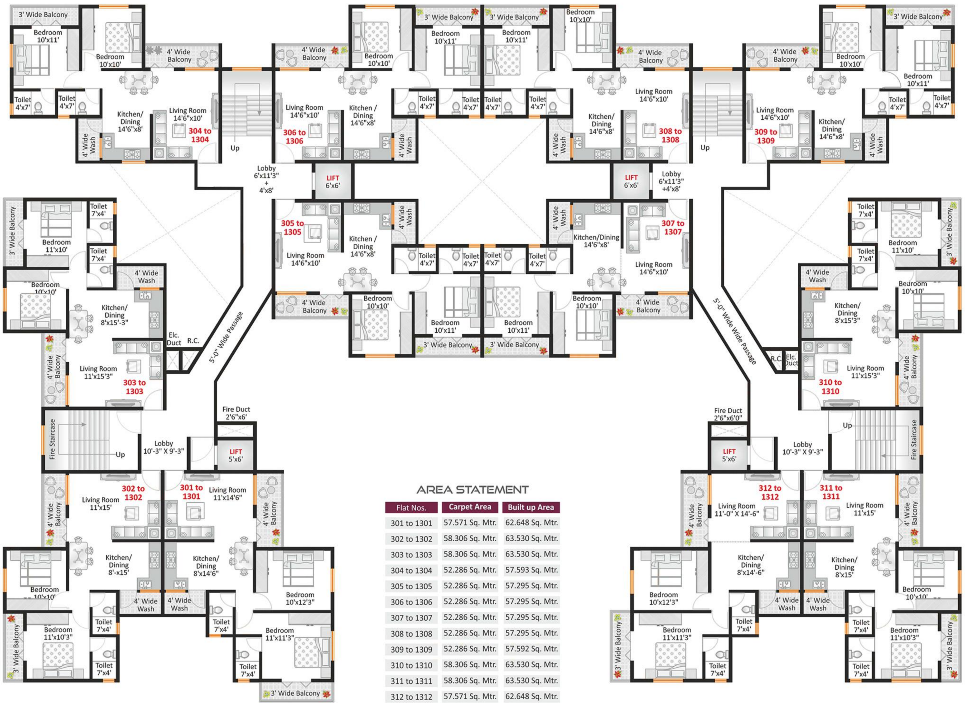
2BHK TYPICAL FLOOR PLAN - WING E & A
