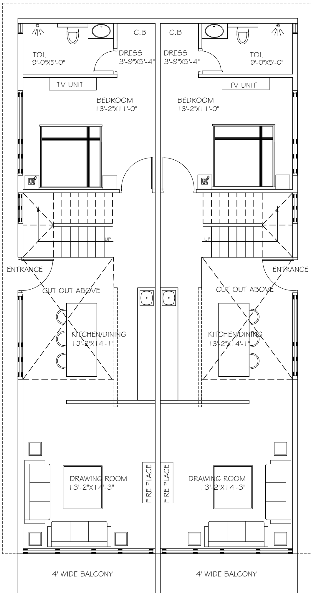
FIRST FLOOR BLOCK 6
