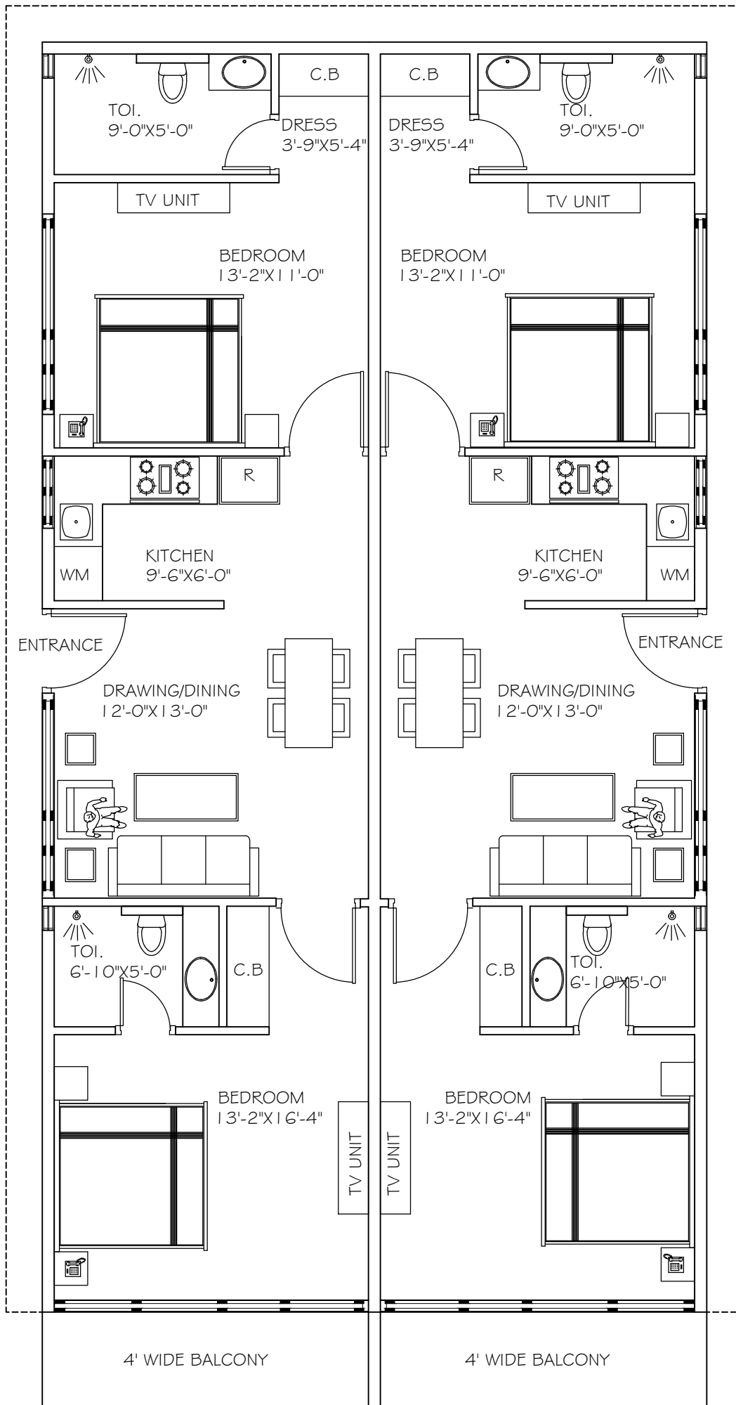
GROUND FLOOR BLOCK 6
