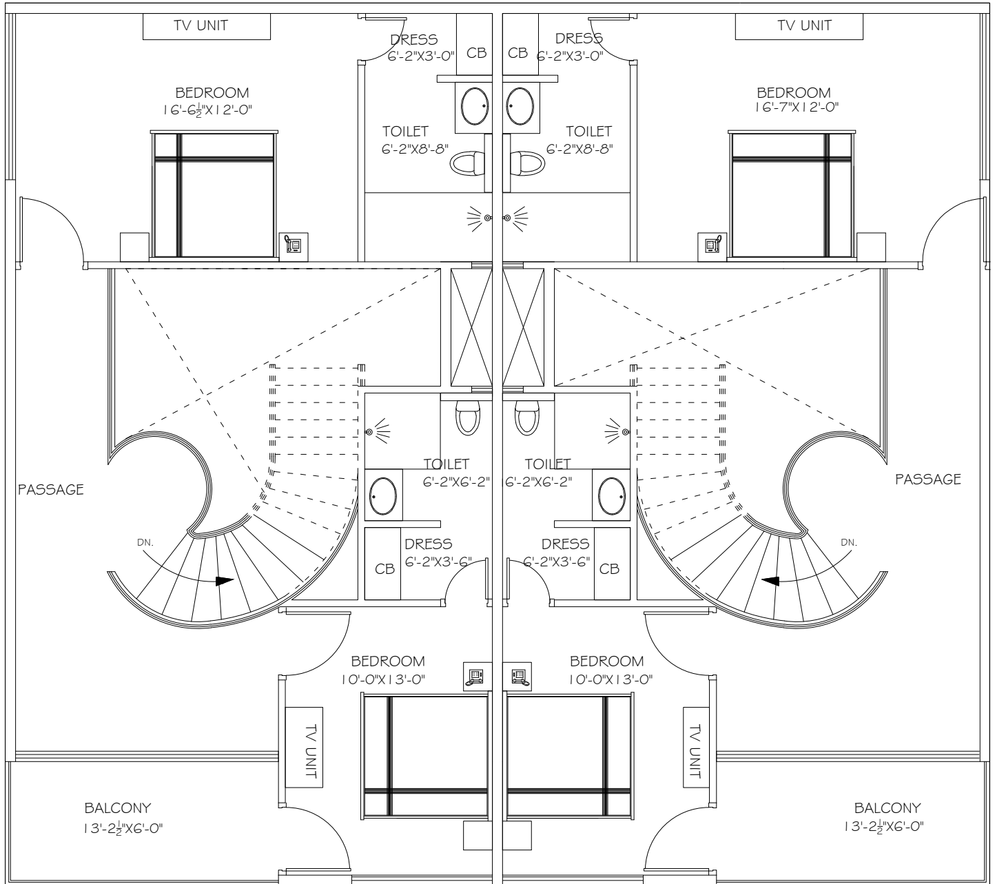
TOP FLOOR
