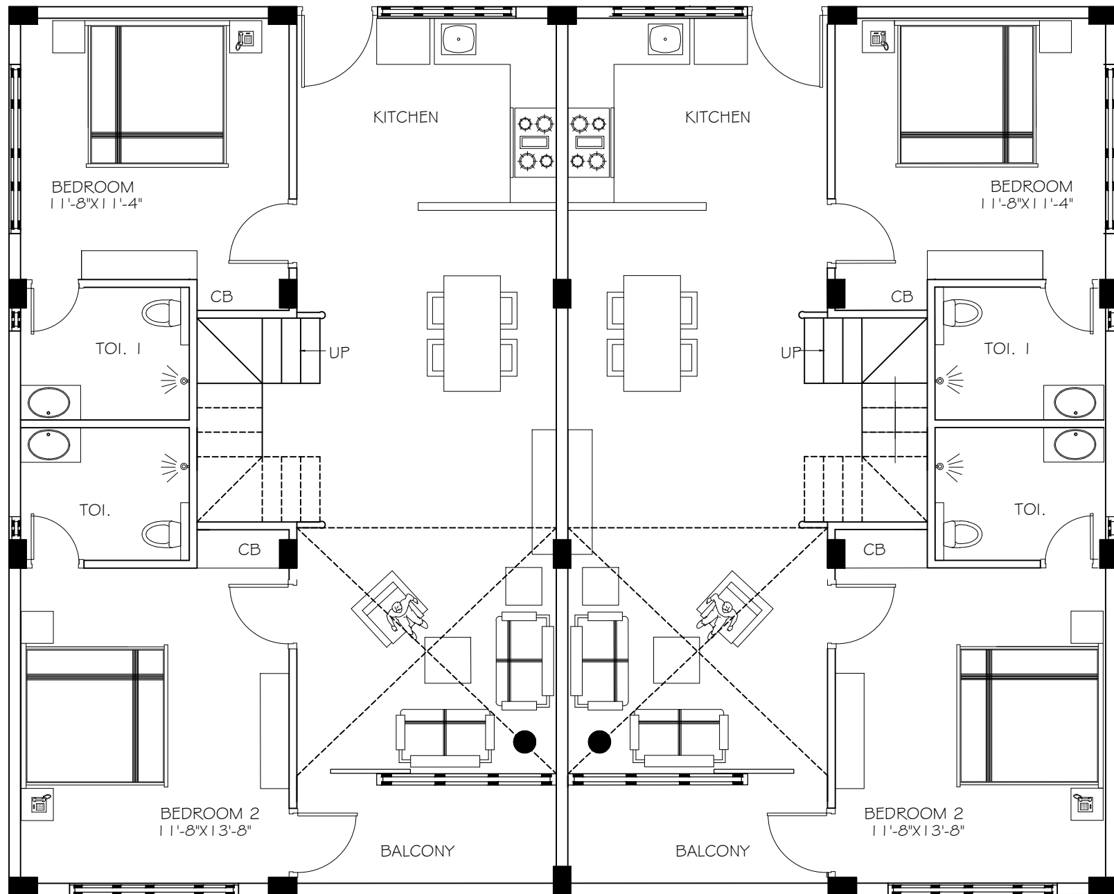
block 8 -duplex lower floor
