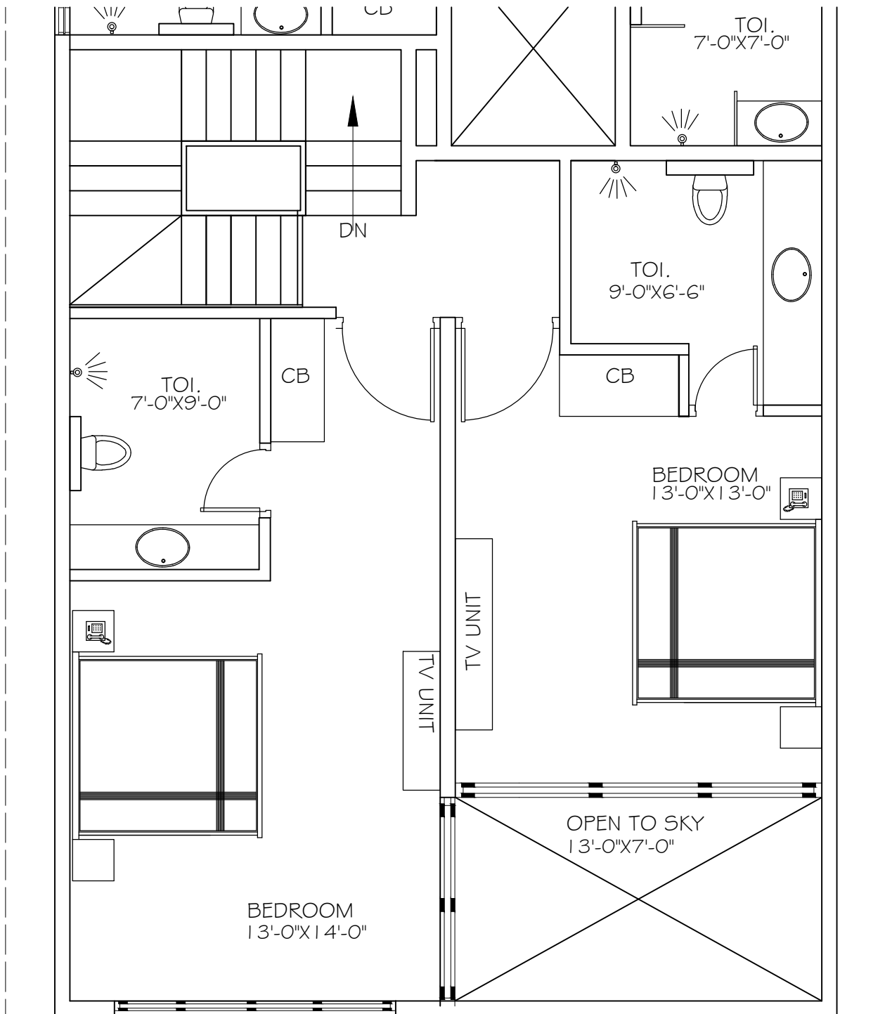
DUPLEX UPPER FLOOR
