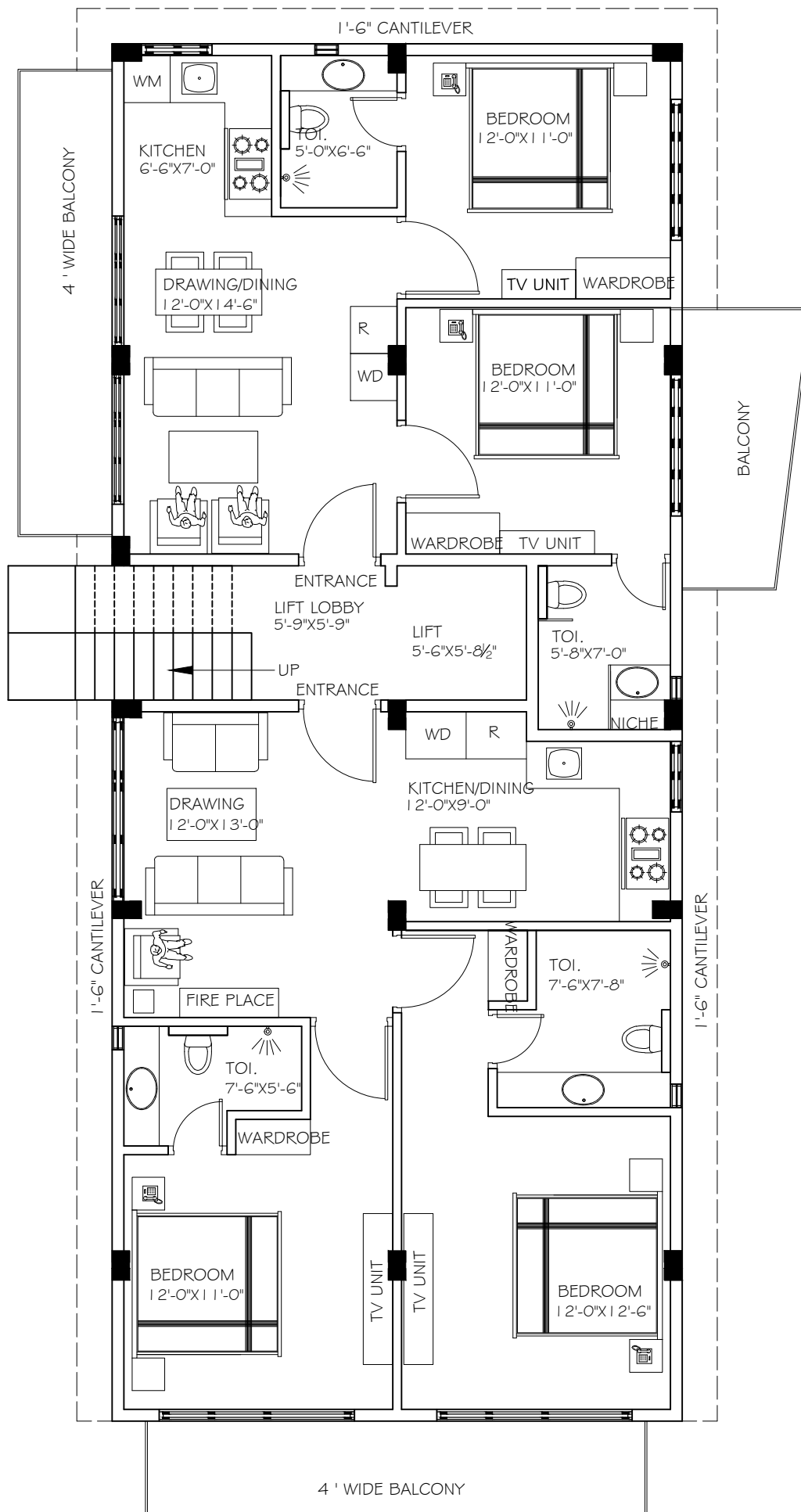
First Floor BLOCK 1
