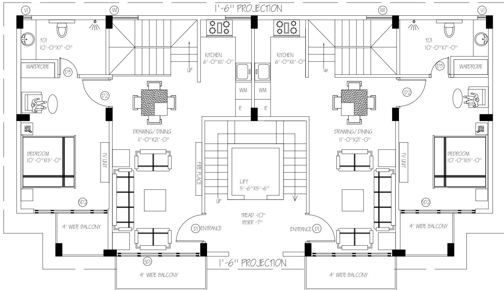
3 BHK DUPLEX-LOWER FLOOR PLAN
