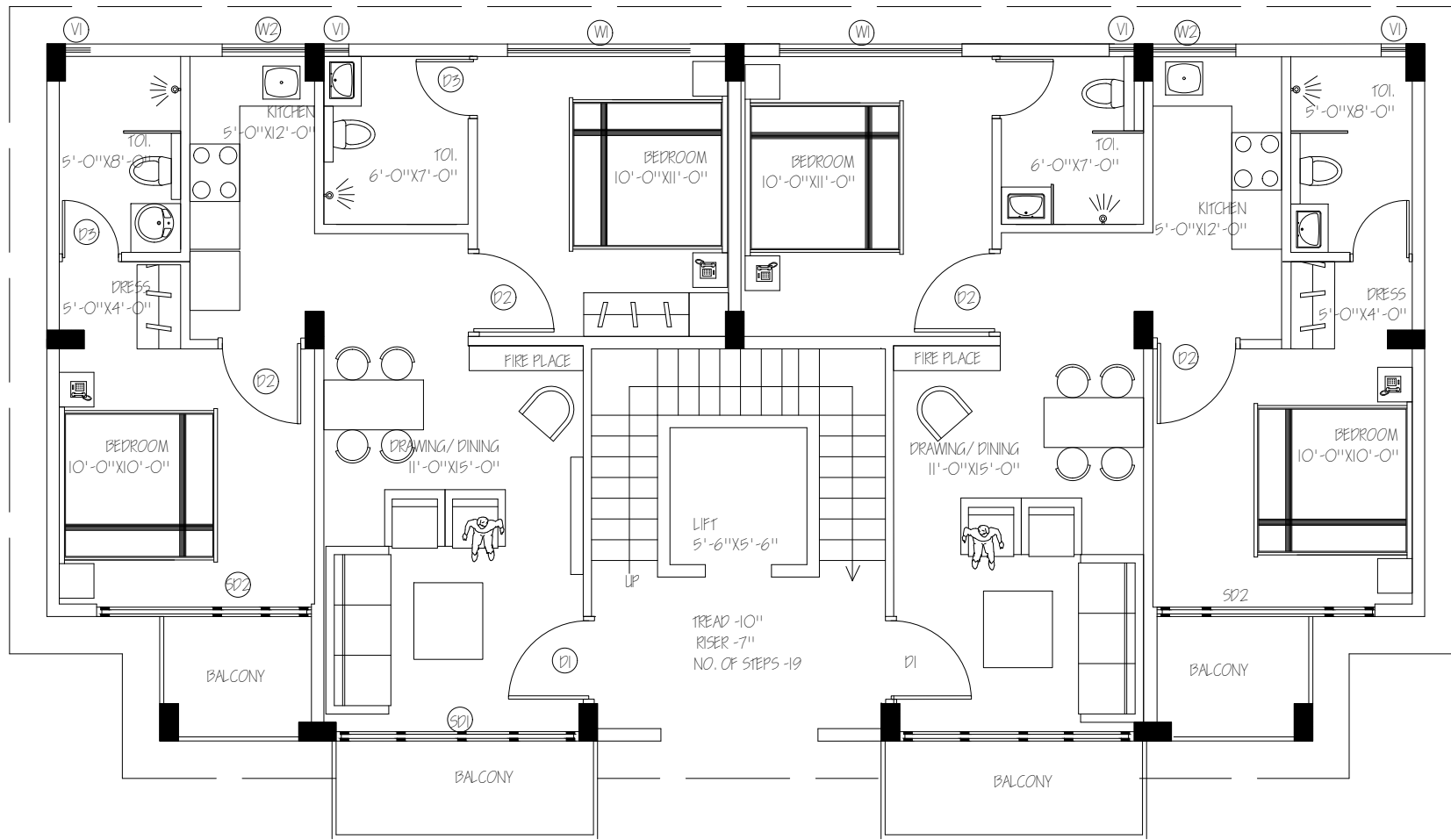
TYPICAL FLOOR PLAN - 2BHK
