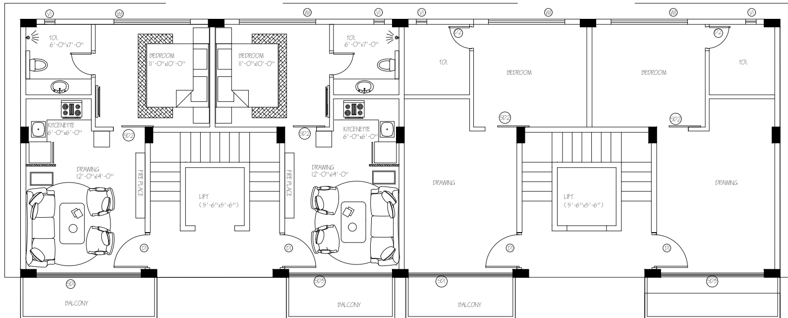
TYPICAL FLOOR PLAN STUDIO
