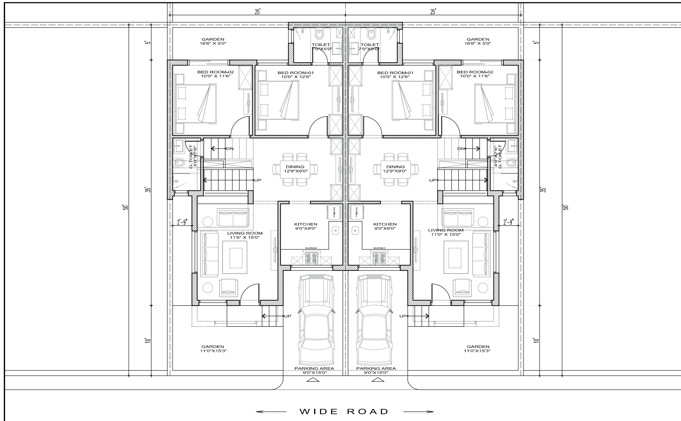
Ground Floor Plan 2BHK Area: 991 Sqft
