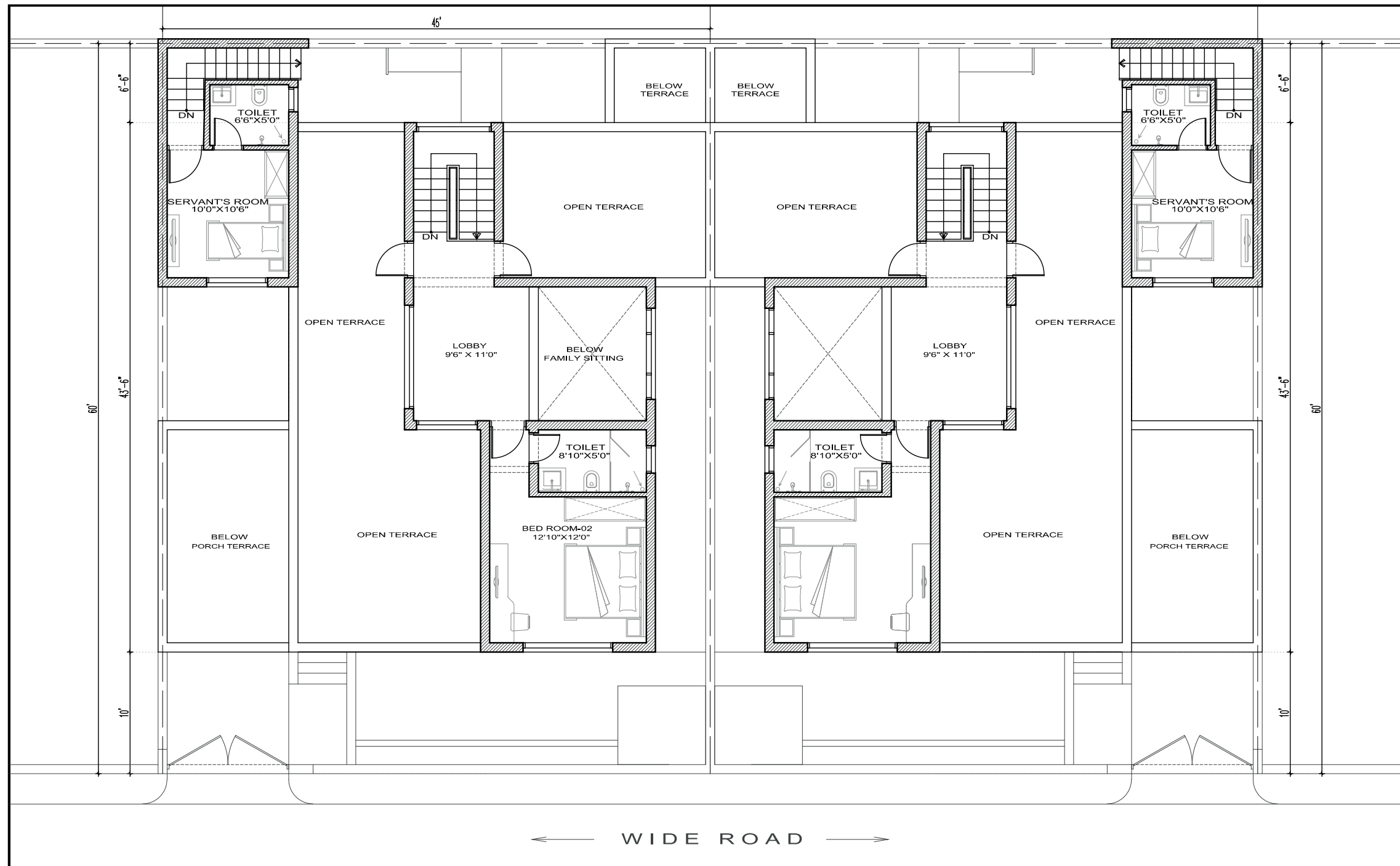
First Floor Plan 3BHK Area: 2153 Sqft
