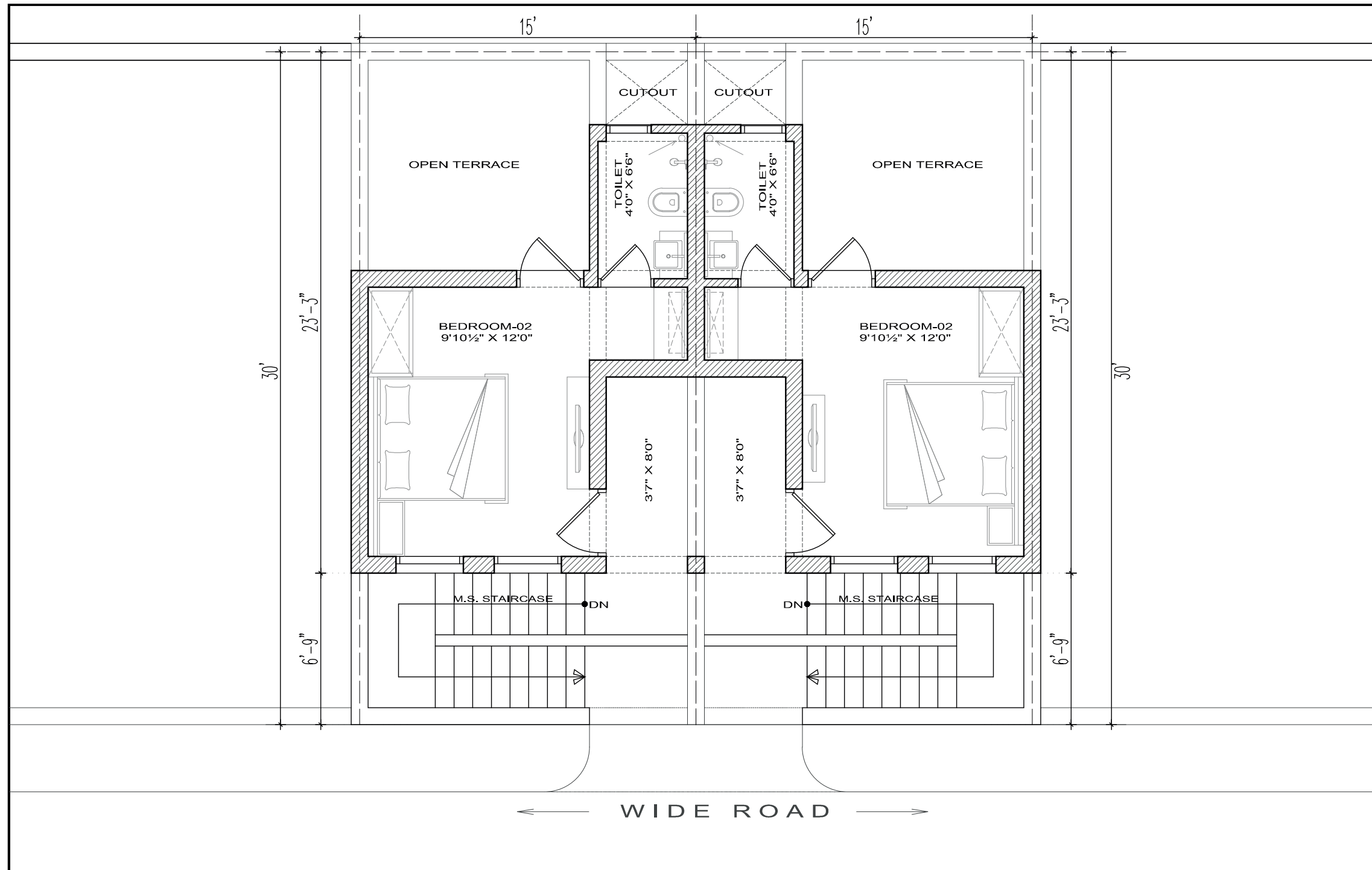
Ground Floor Plan 2BHK Area: 603 Sqft
