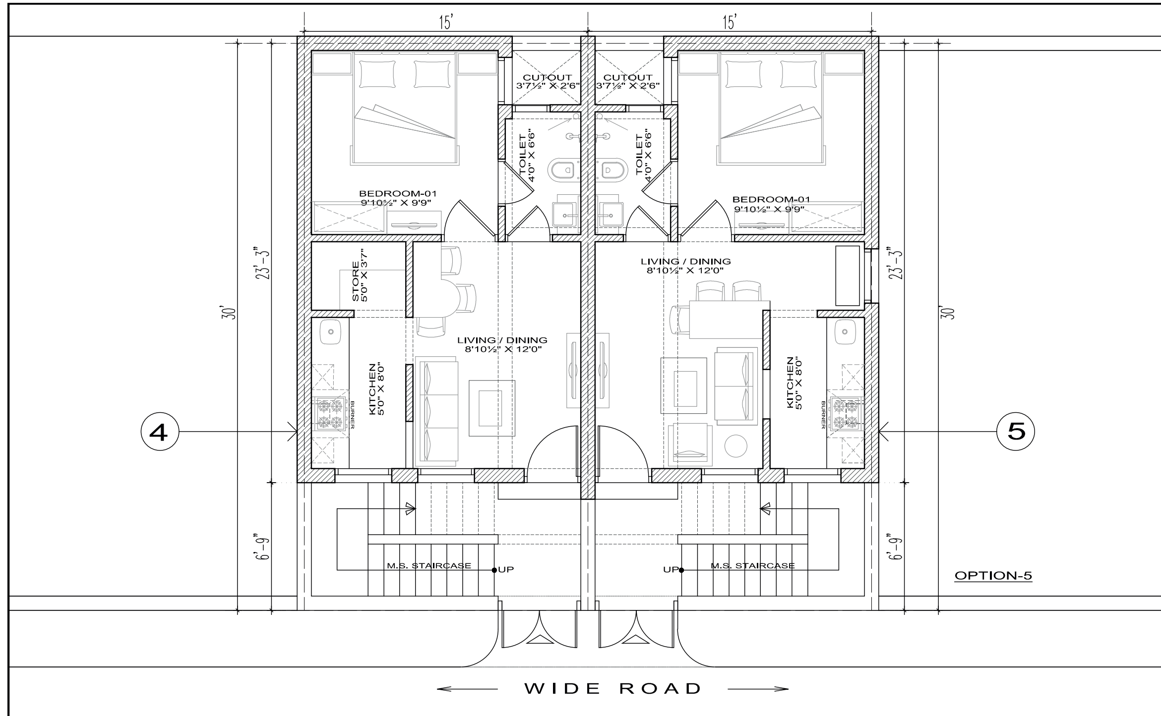
Ground Floor Plan 1BHK Area: 405 Sqft
