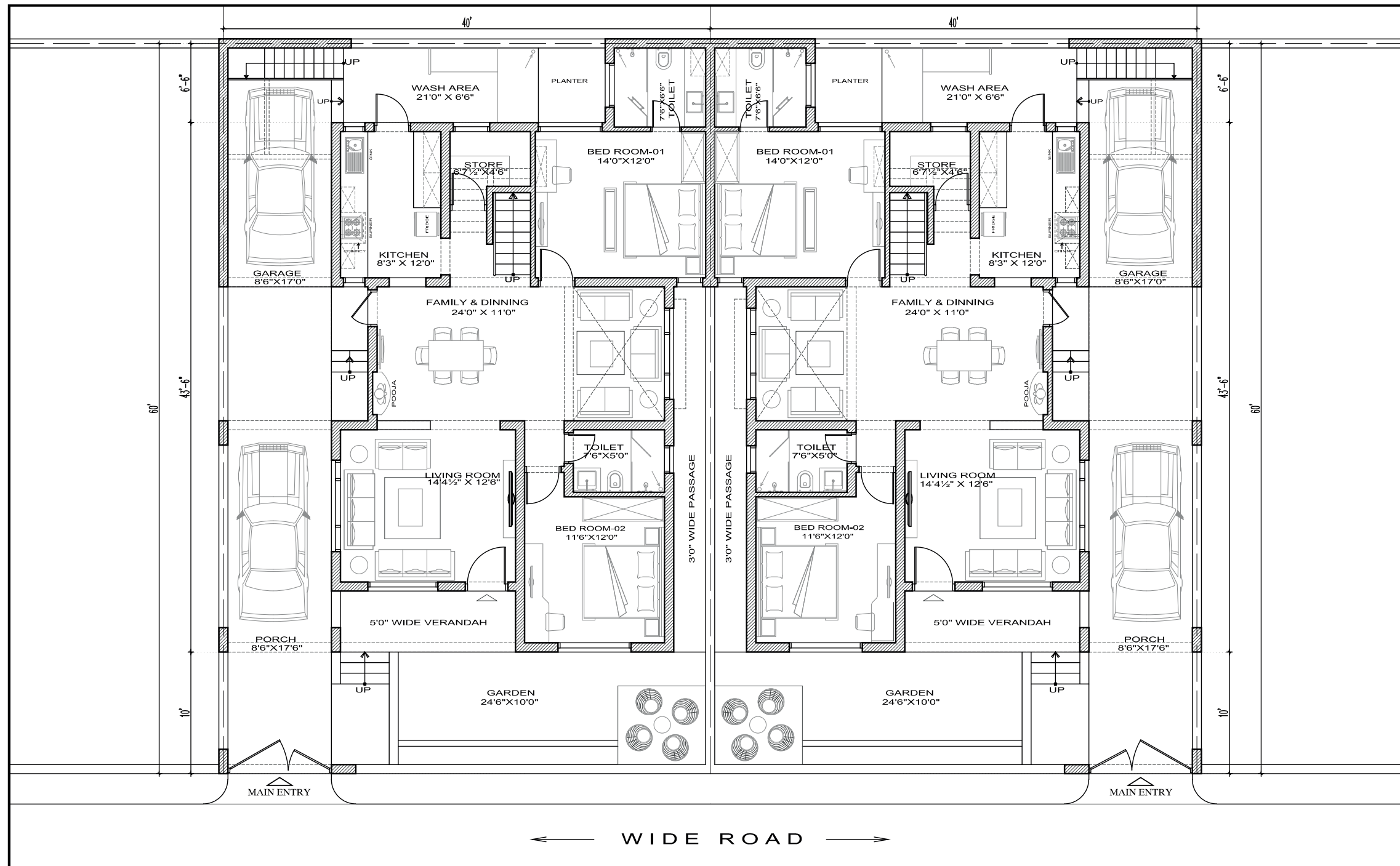
Ground Floor Plan 3BHK Area: 1986 Sqft
