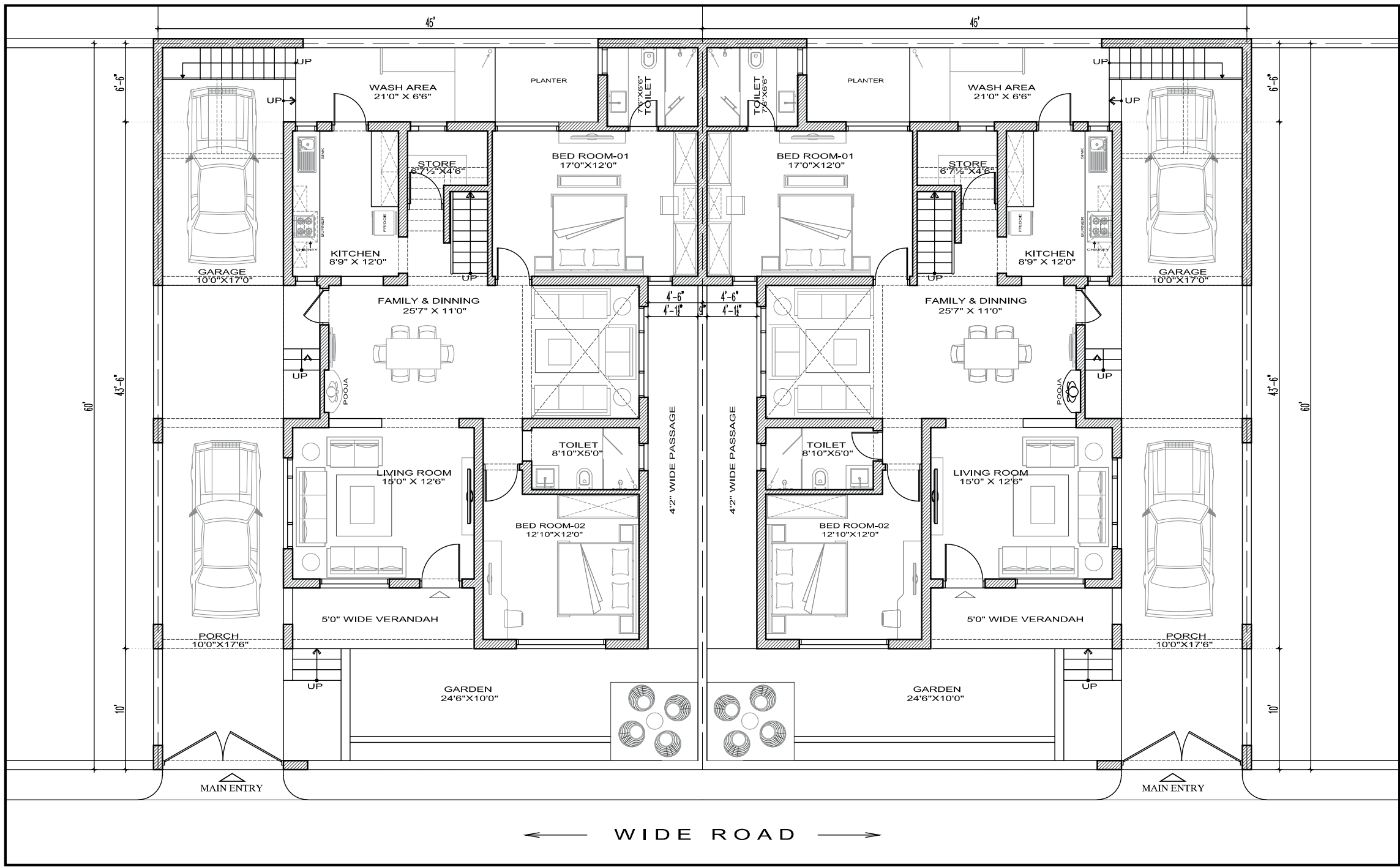
Ground Floor Plan 3BHK Area: 2153 Sqft
