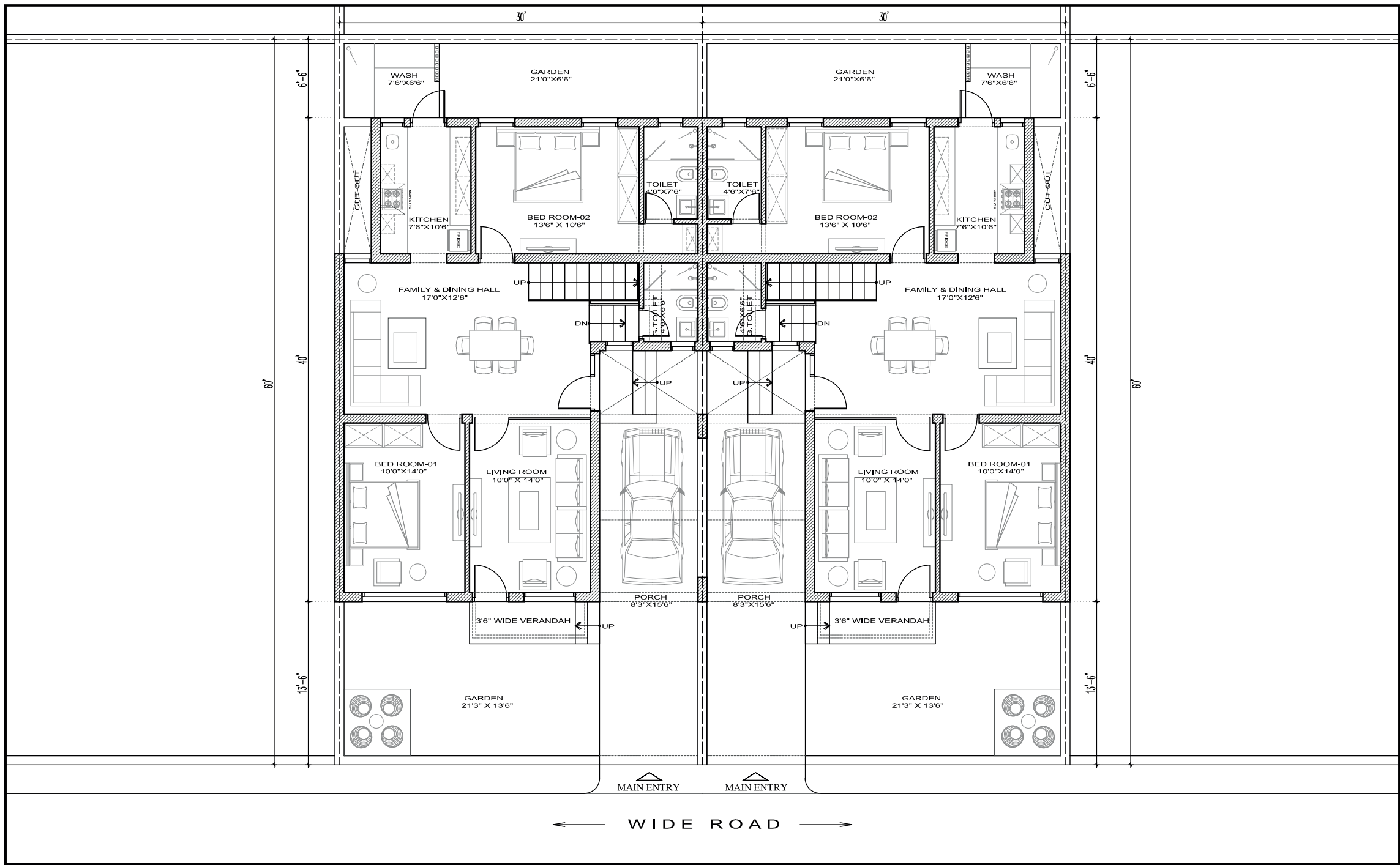
Ground Floor Plan 2BHK Area: 1298 Sqft
