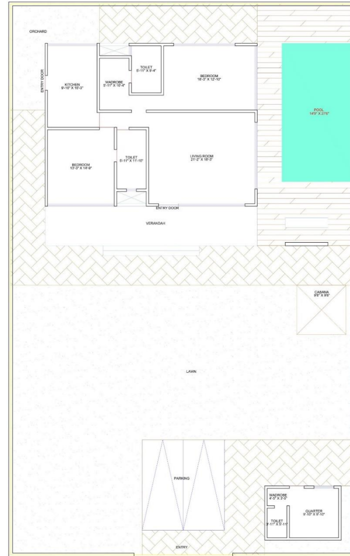
7500 SQ. FT. COTTAGE PLAN
