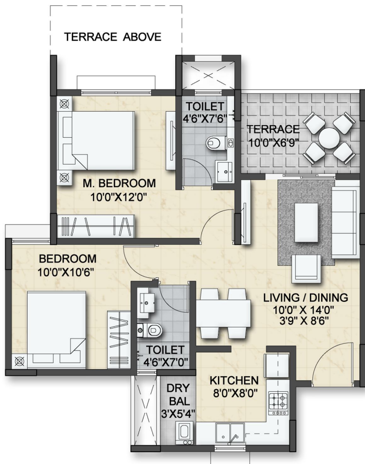
ODD FLOOR UNIT PLAN
