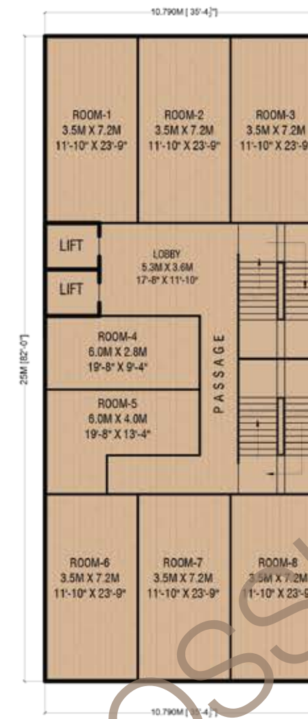
2ND / 3RD / 4TH / 5TH / 6TH / 7TH / 8TH TYPICAL FLOOR PLAN [HOTEL ROOM = 7 X 6 = 56 ROOMS]
