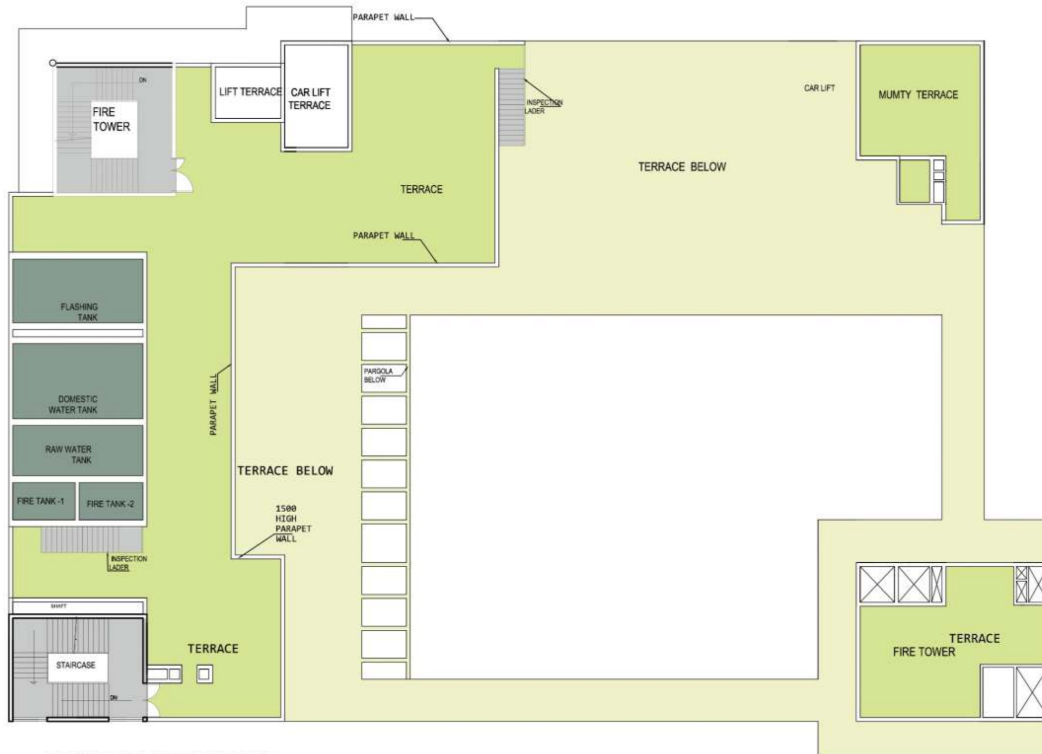
TERRACE FLOOR LVL PLAN
