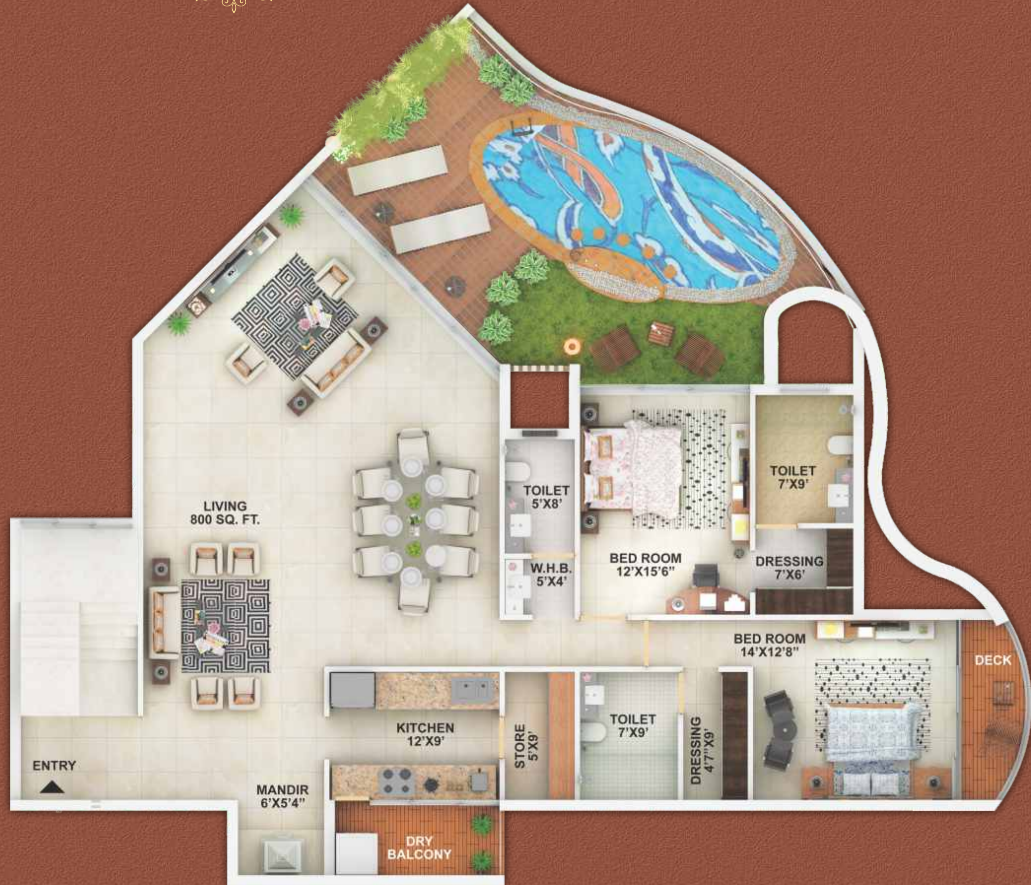
Duplex 2D Lower Floor Plan (2885 sq. ft.) ★★★★★
