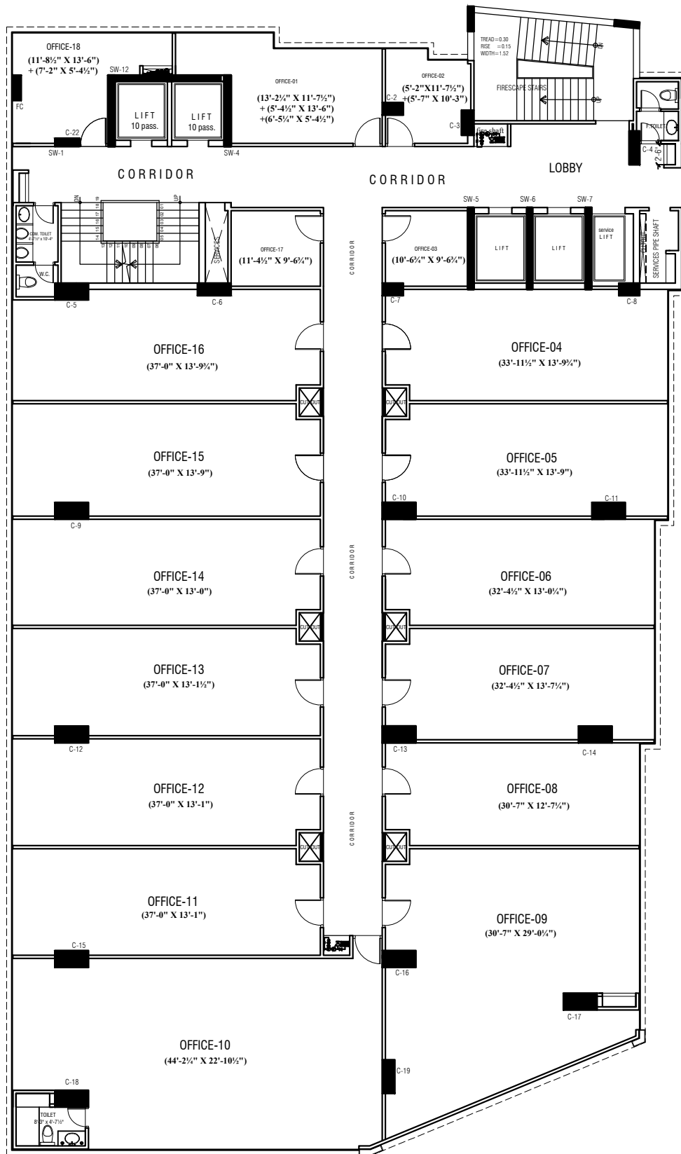
6th FLOOR PLAN
