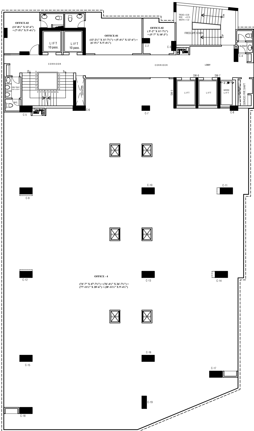
10th, 11th & 12th FLOOR PLAN
