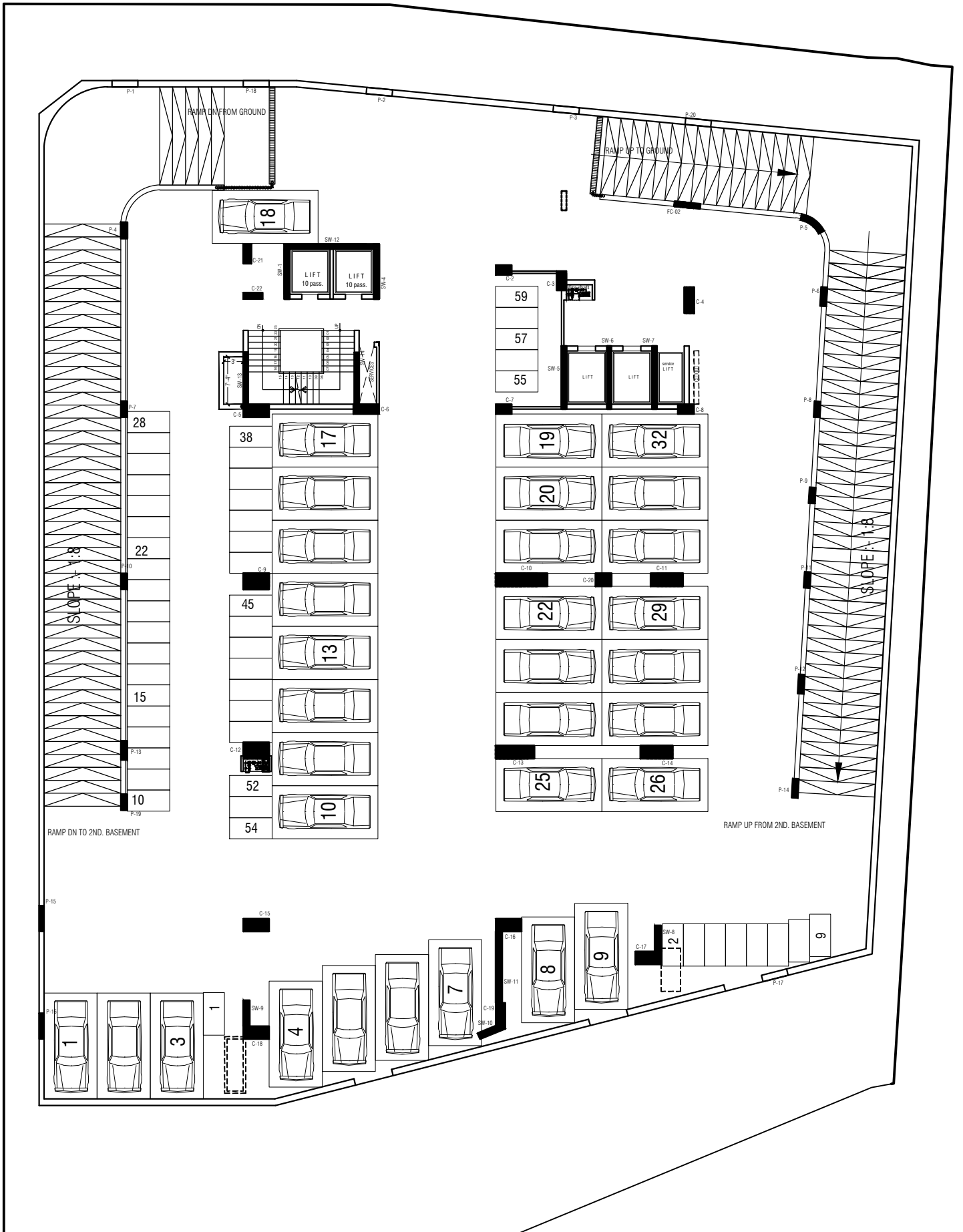
BASEMENT -1 FLOOR PLAN
