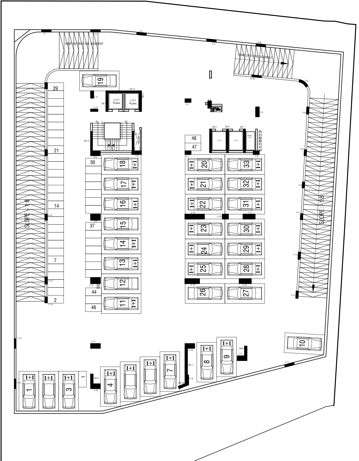
BASEMENT -3 FLOOR PLAN
