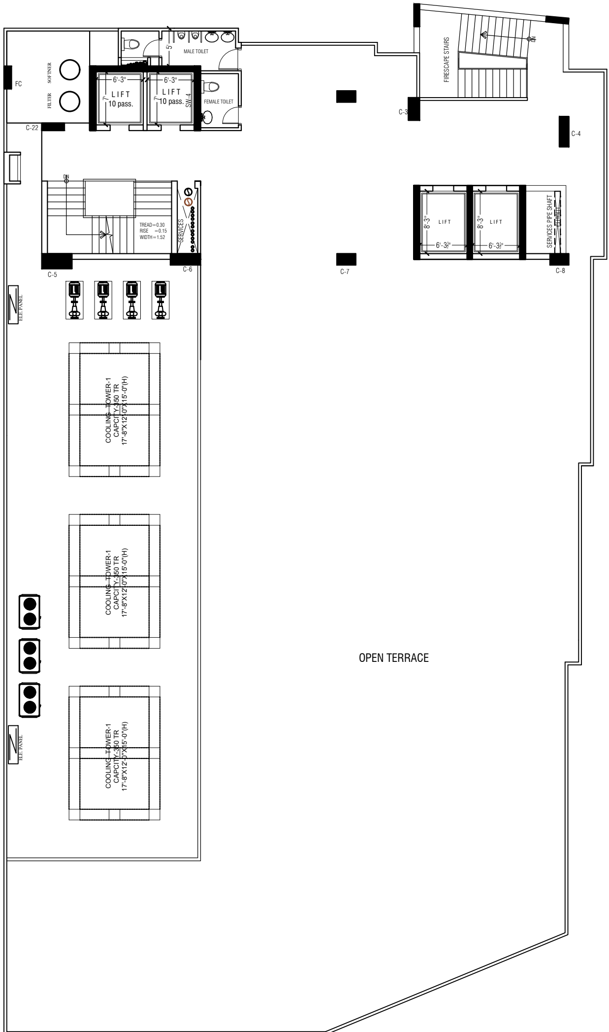
TERRACE LOWER LEVEL PLAN
