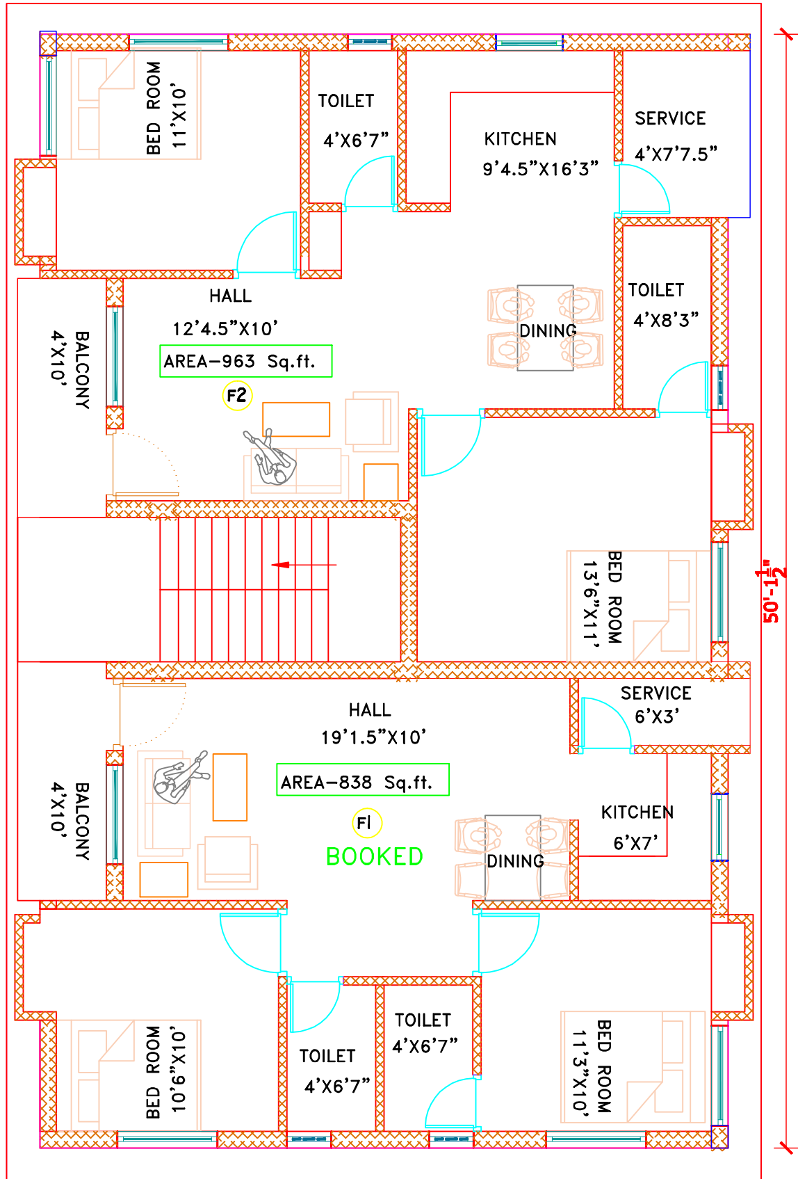
ROAD FIRST FLOOR PLAN PROPOSED APARTMENT VENGAI VASAL
