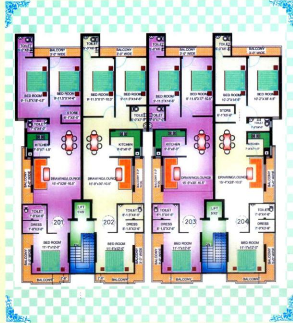
First & Second Floor Plan
