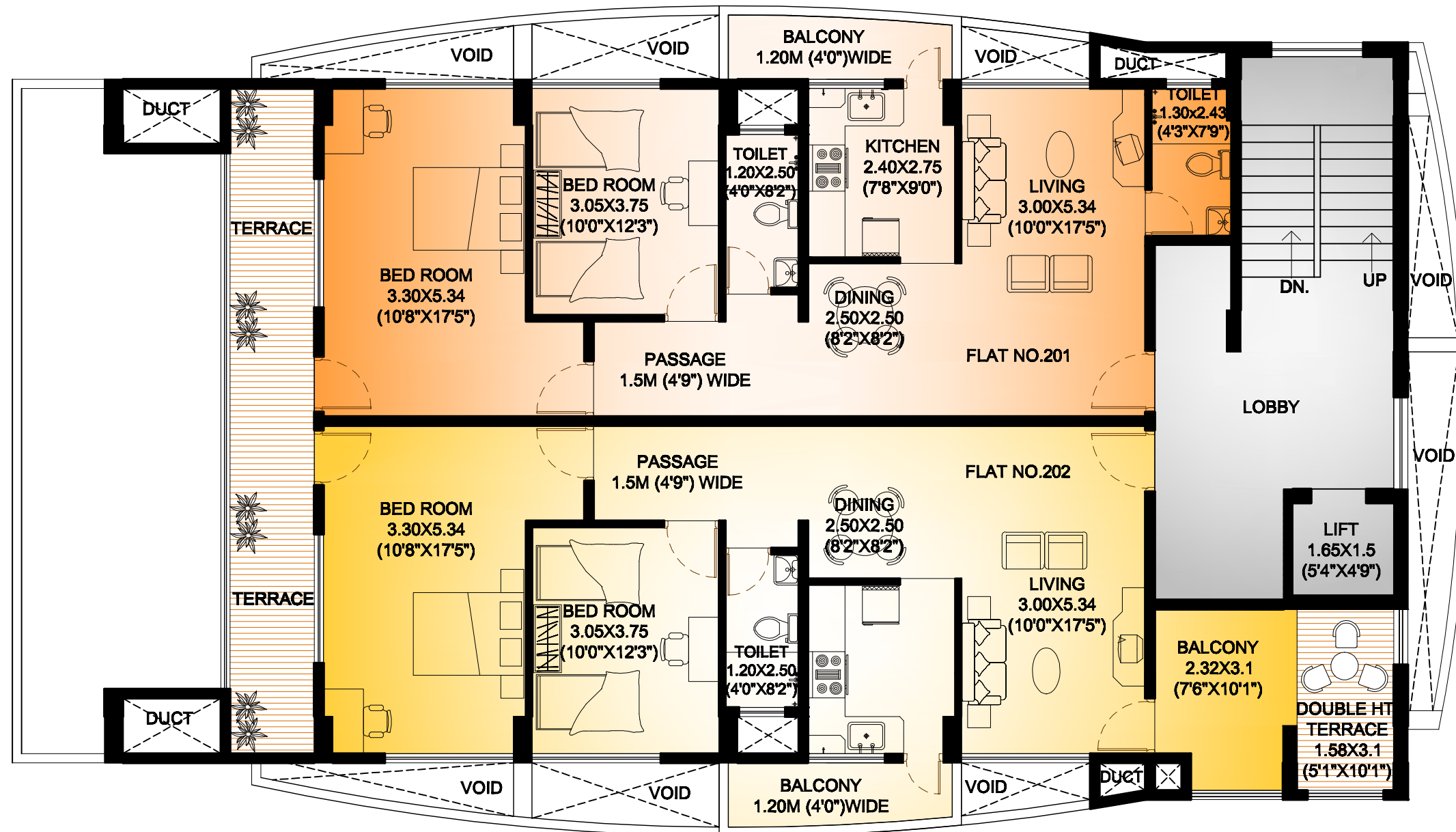
Illrd FLOOR PLAN
