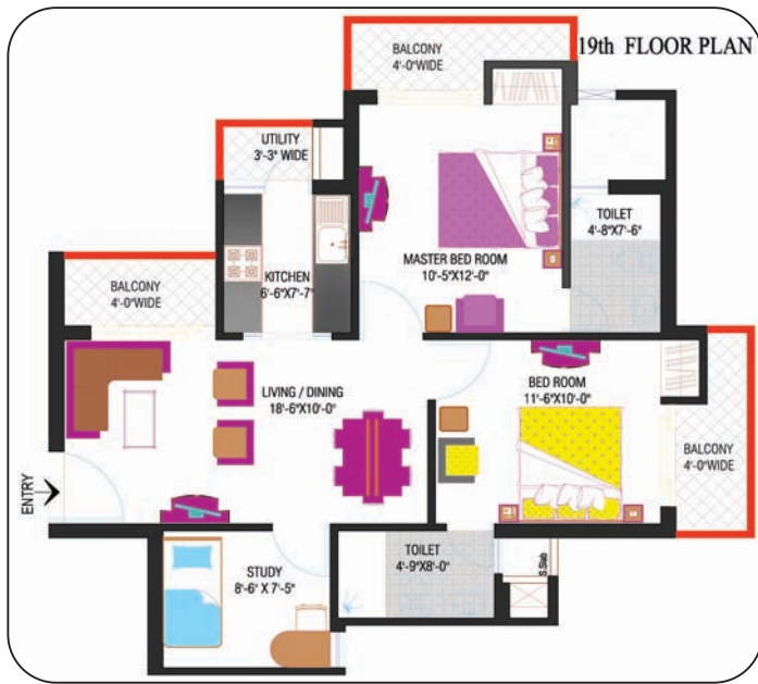
KEY PLAN (TOWER-G, K, M, P & Q) 2 BED + 2 TOILET UNIT + STUDY
