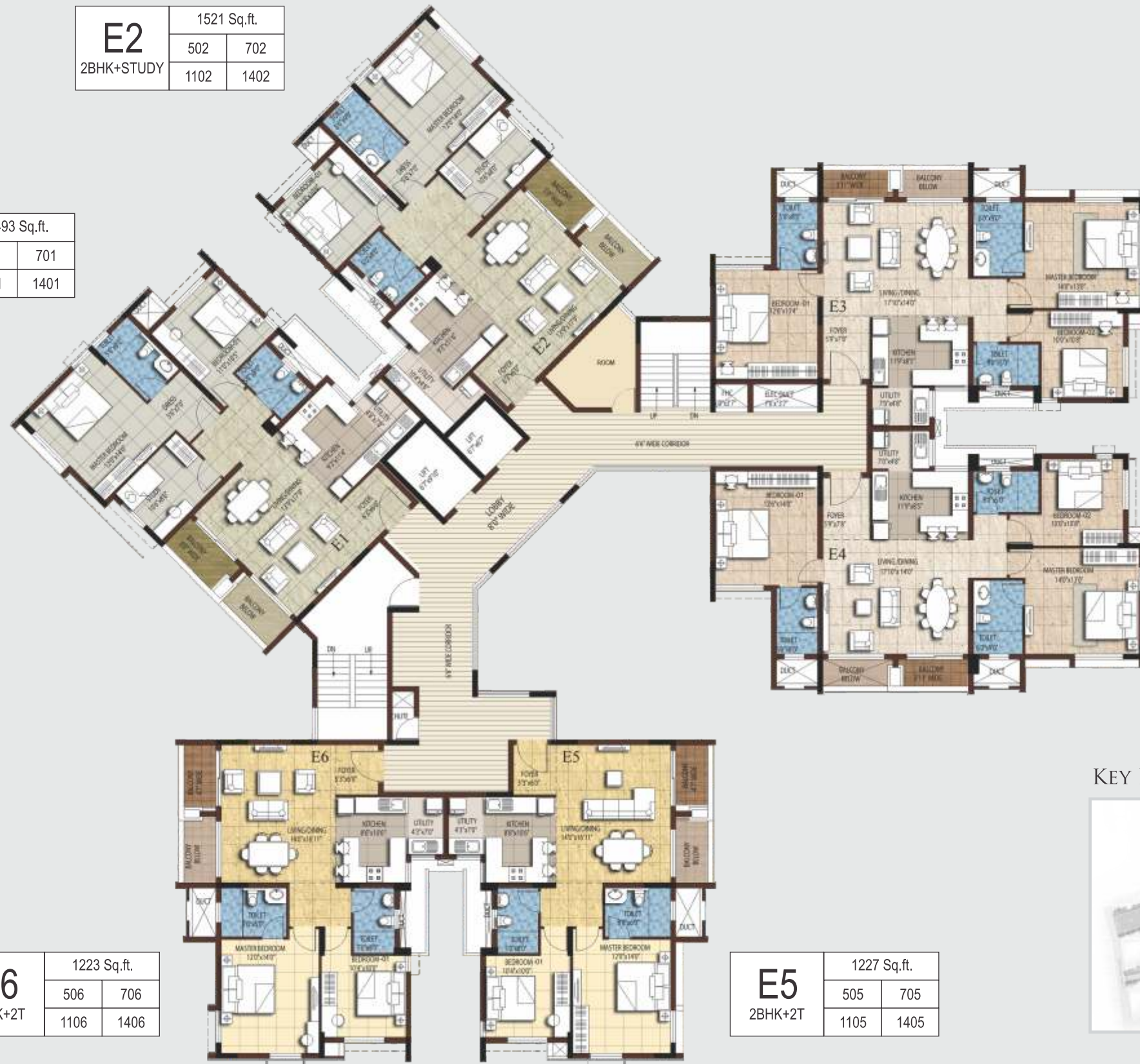
TOWER E 5 TH , 7 TH , 11 TH & 14 TH FLOOR PLAN
