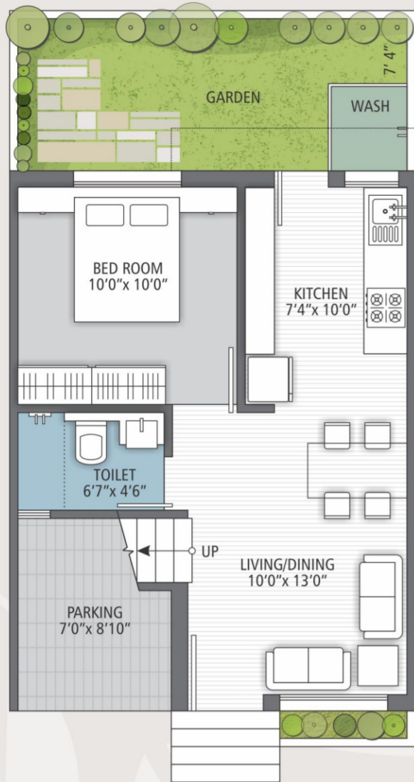
GROUND FLOOR PLAN Built up Area: 505 sq.ft. Plot Area: 598 sq.ft.
