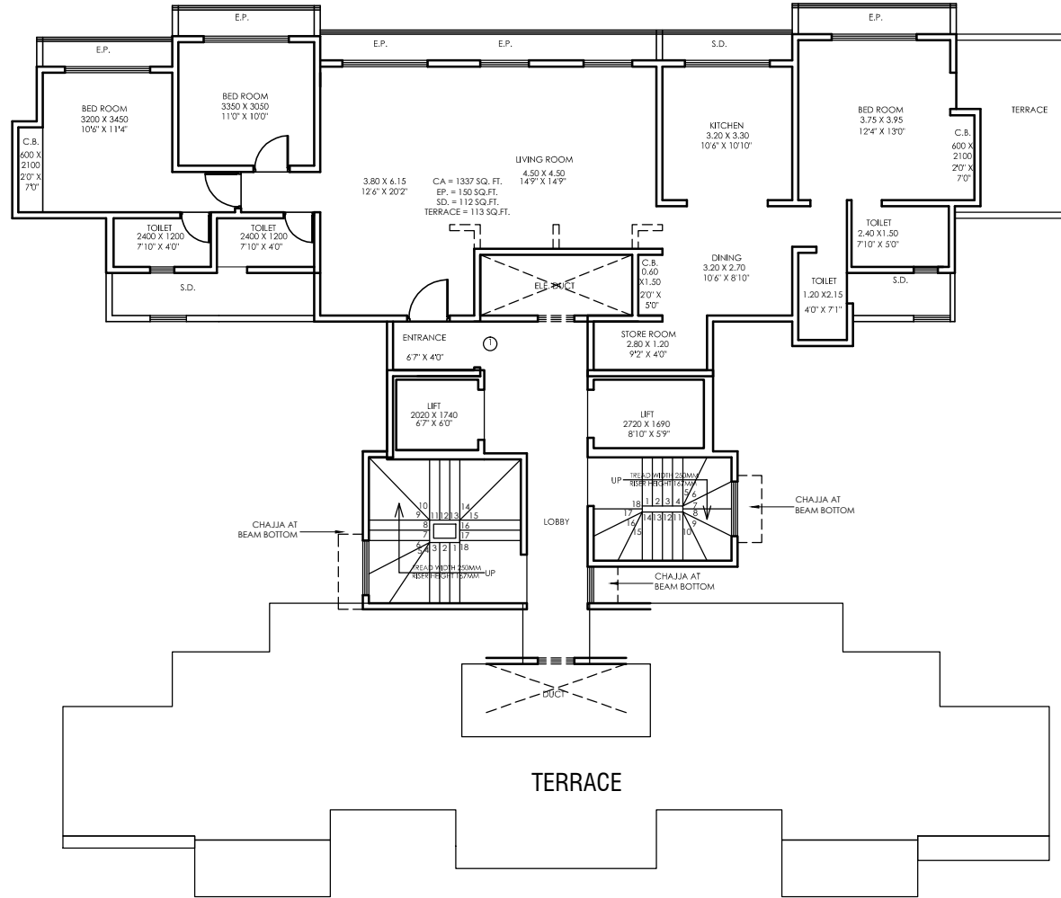
18TH FLOOR PLAN
