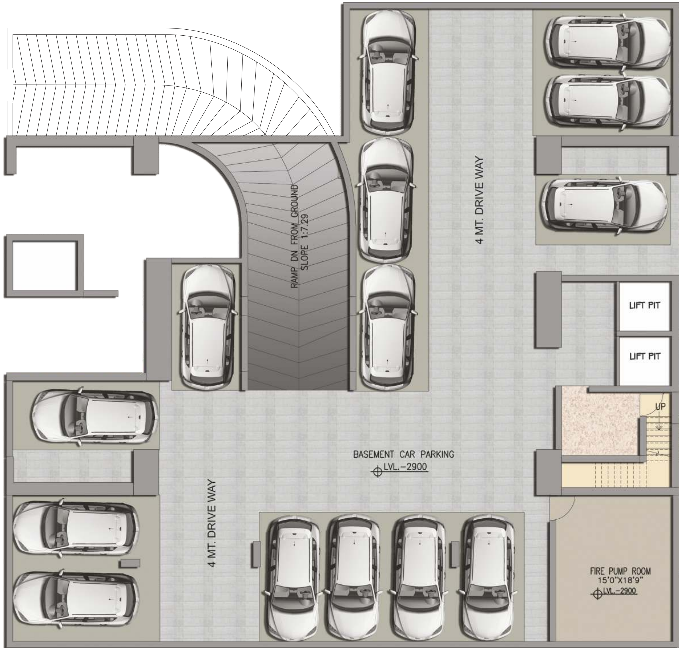
BASEMENT PLAN
