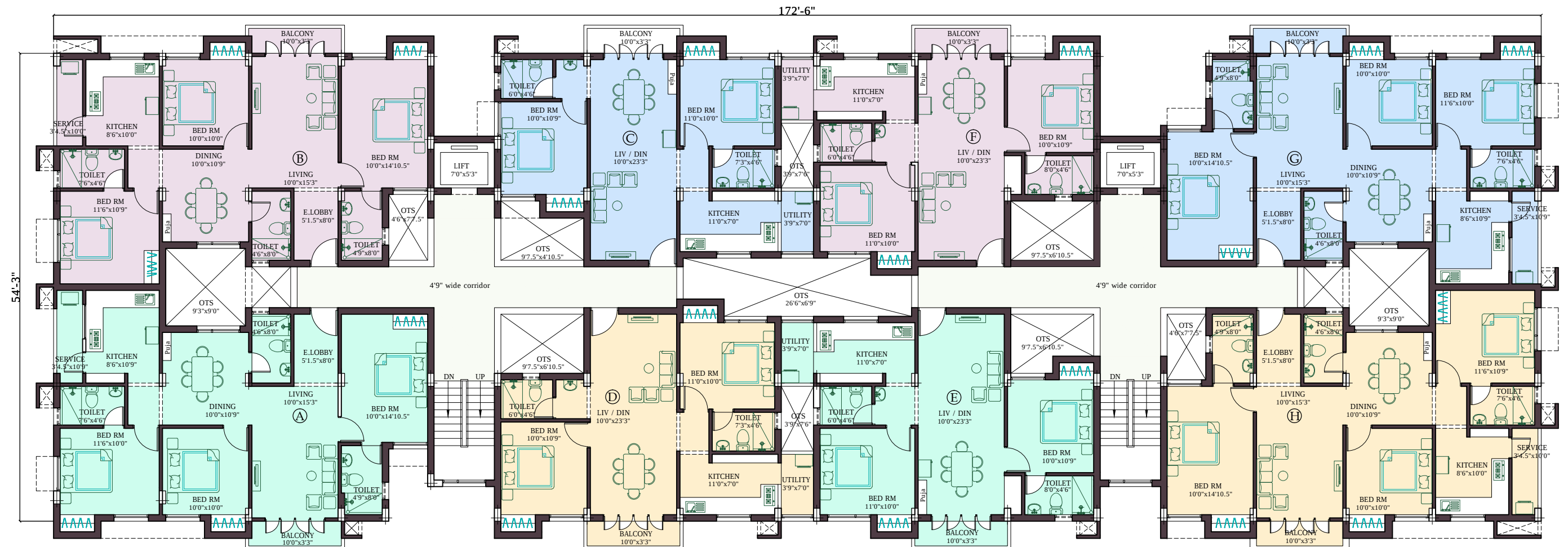
FIRST FLOOR PLAN BLOCK - B
