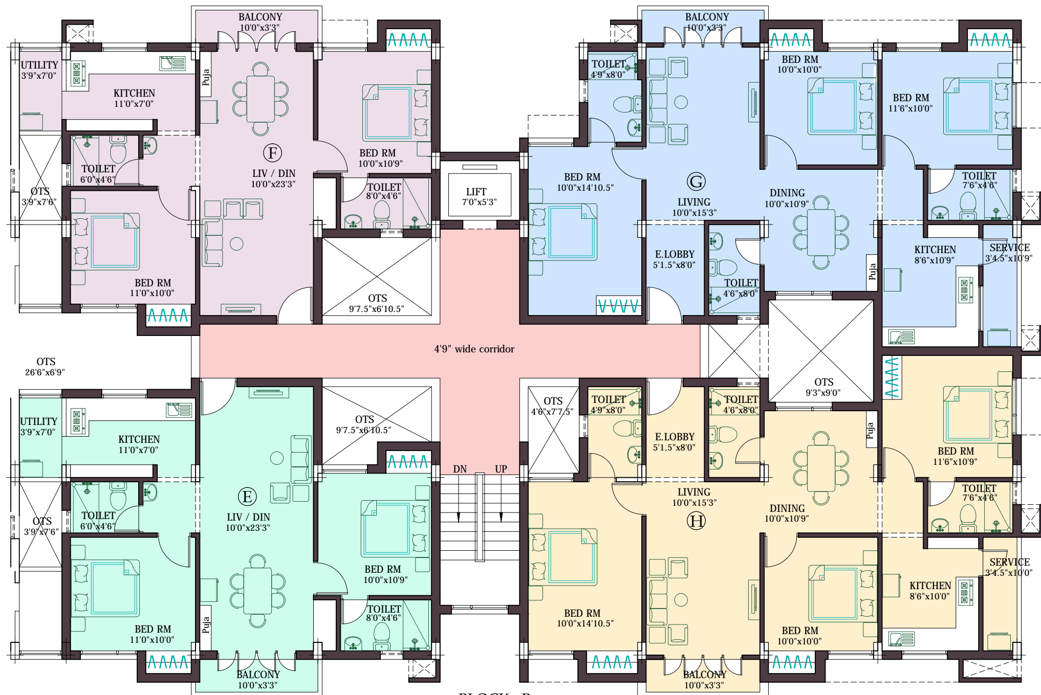
BLOCK - B
