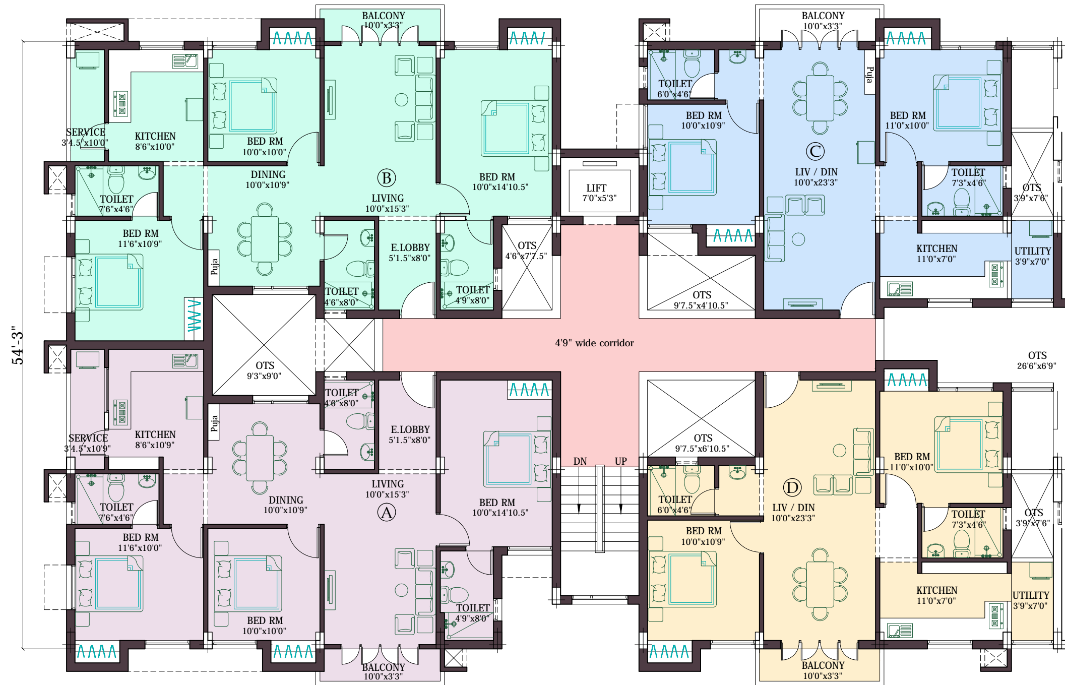
BLOCK - A TYPICAL FLOOR PLAN ( 2nd, 3rd & 4th floor)
