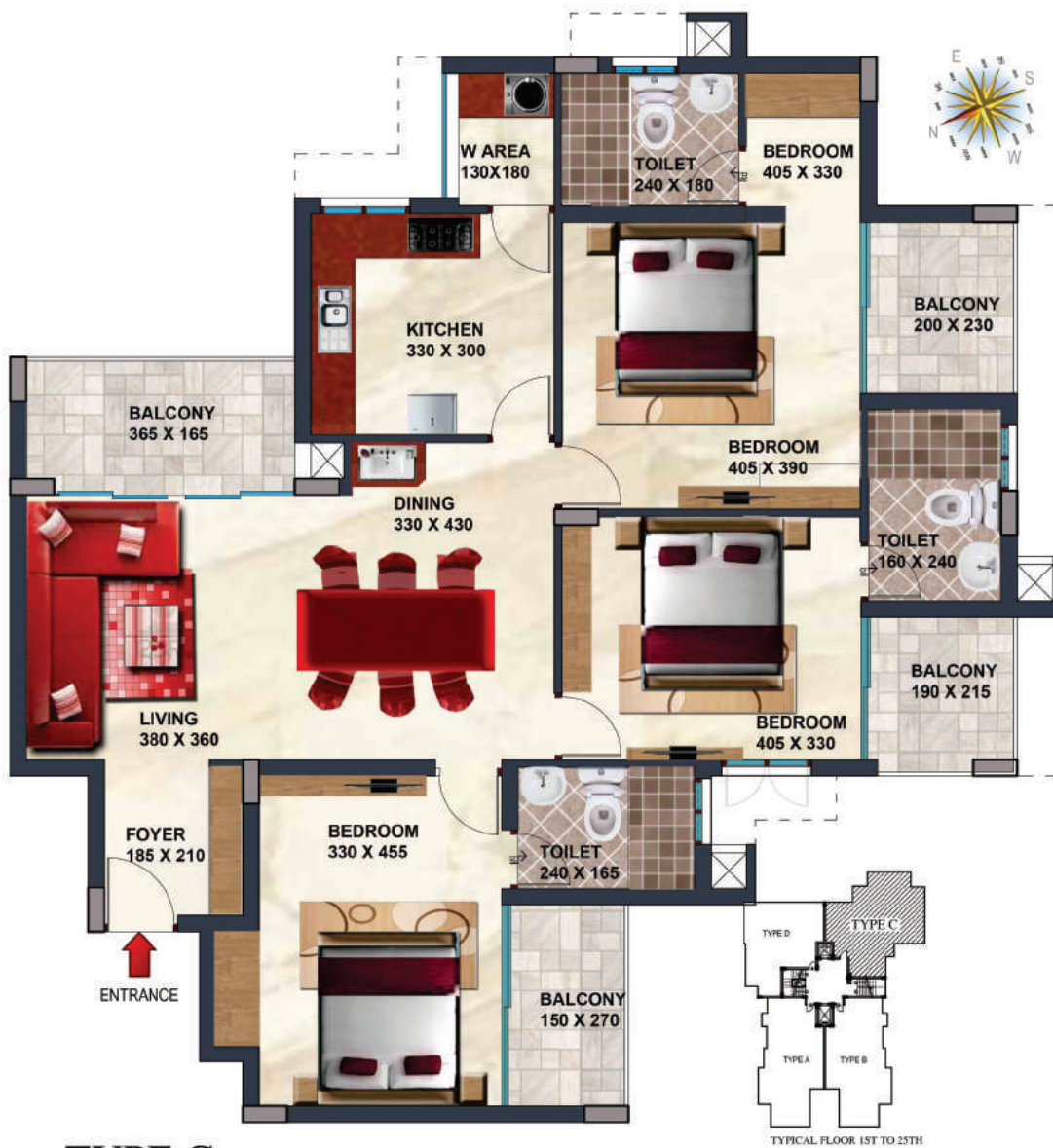
TYPE C SUPER BUILT UP AREA 1905 SQFT
