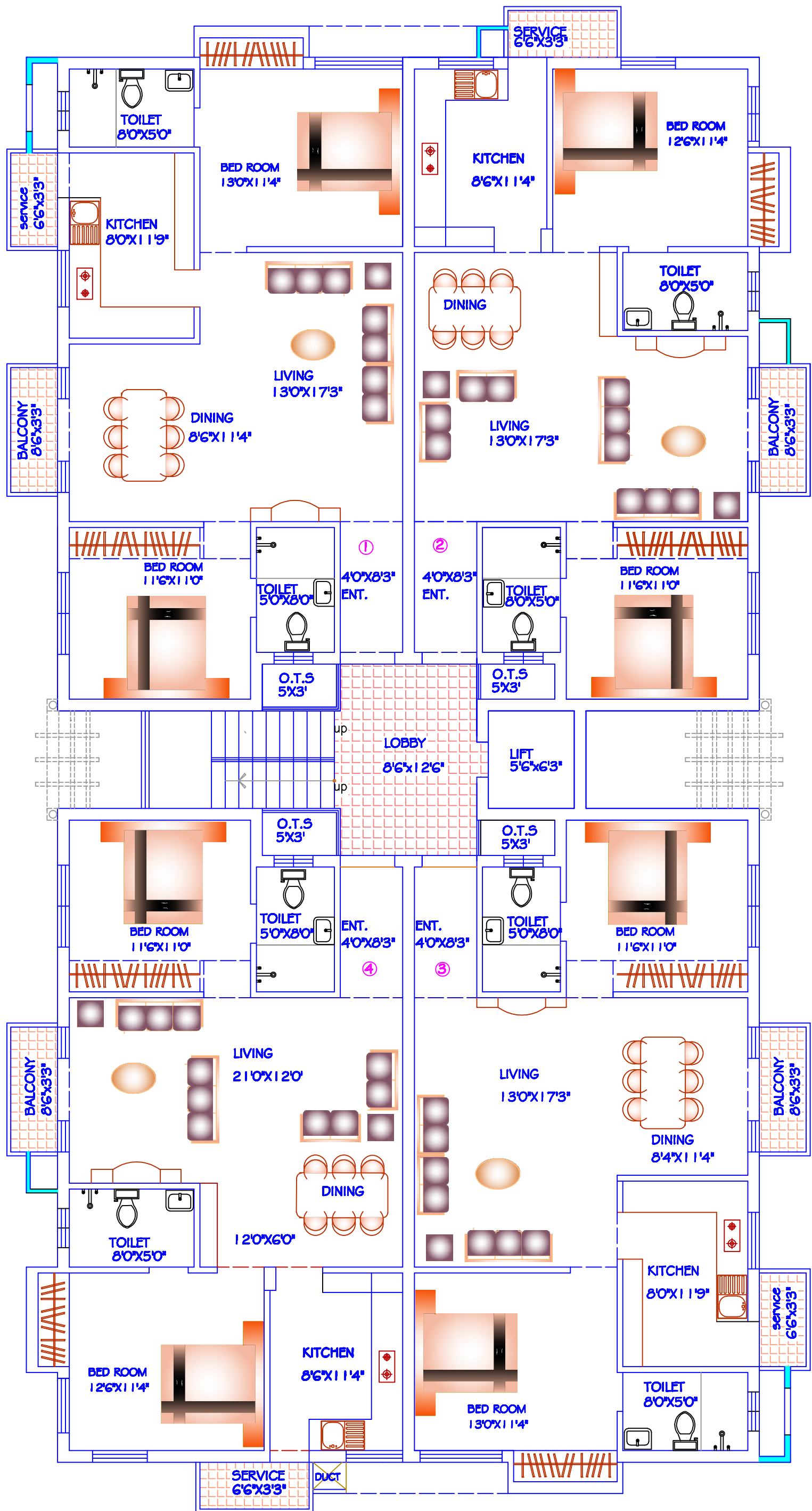
TYPICAL FLOOR PLAN 1st,2nd,3rd& 4th
