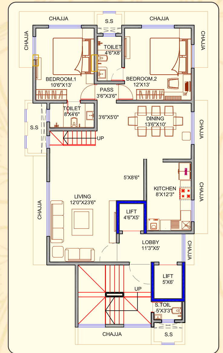
6TH & 13TH, DUPLEX - LOWER LEVEL FLOOR PLAN
