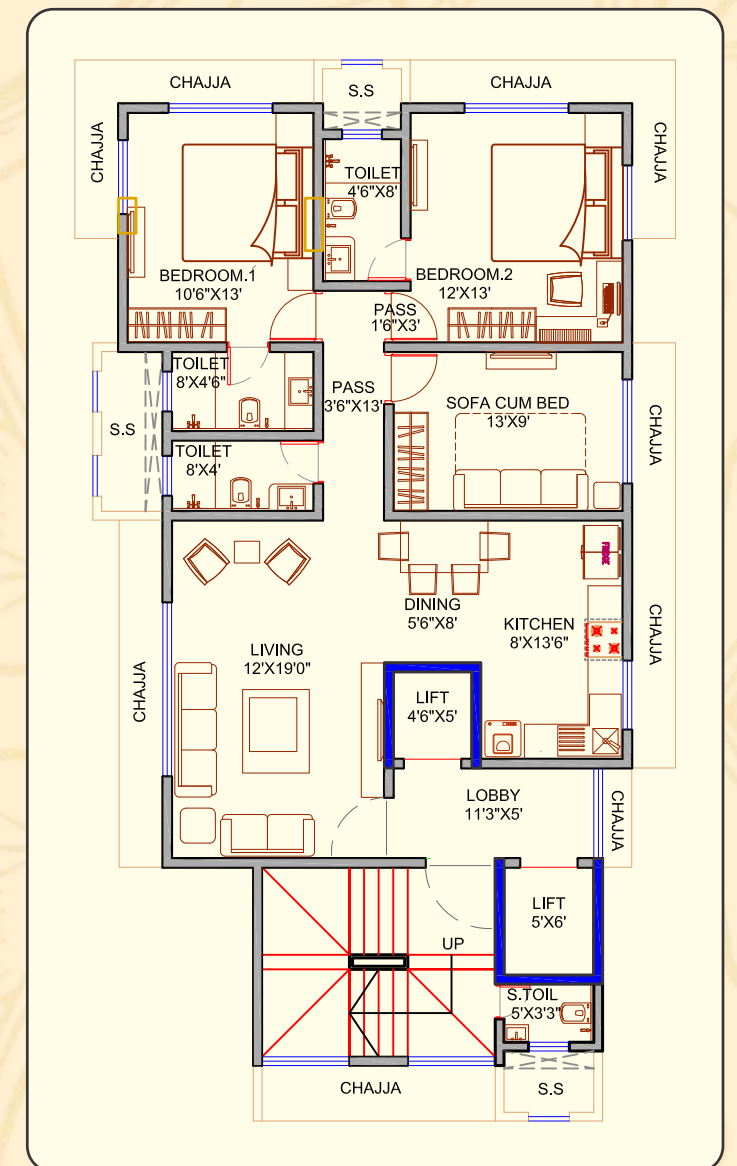
2ND TO 5TH, 8TH TO 12TH FLOOR PLAN
