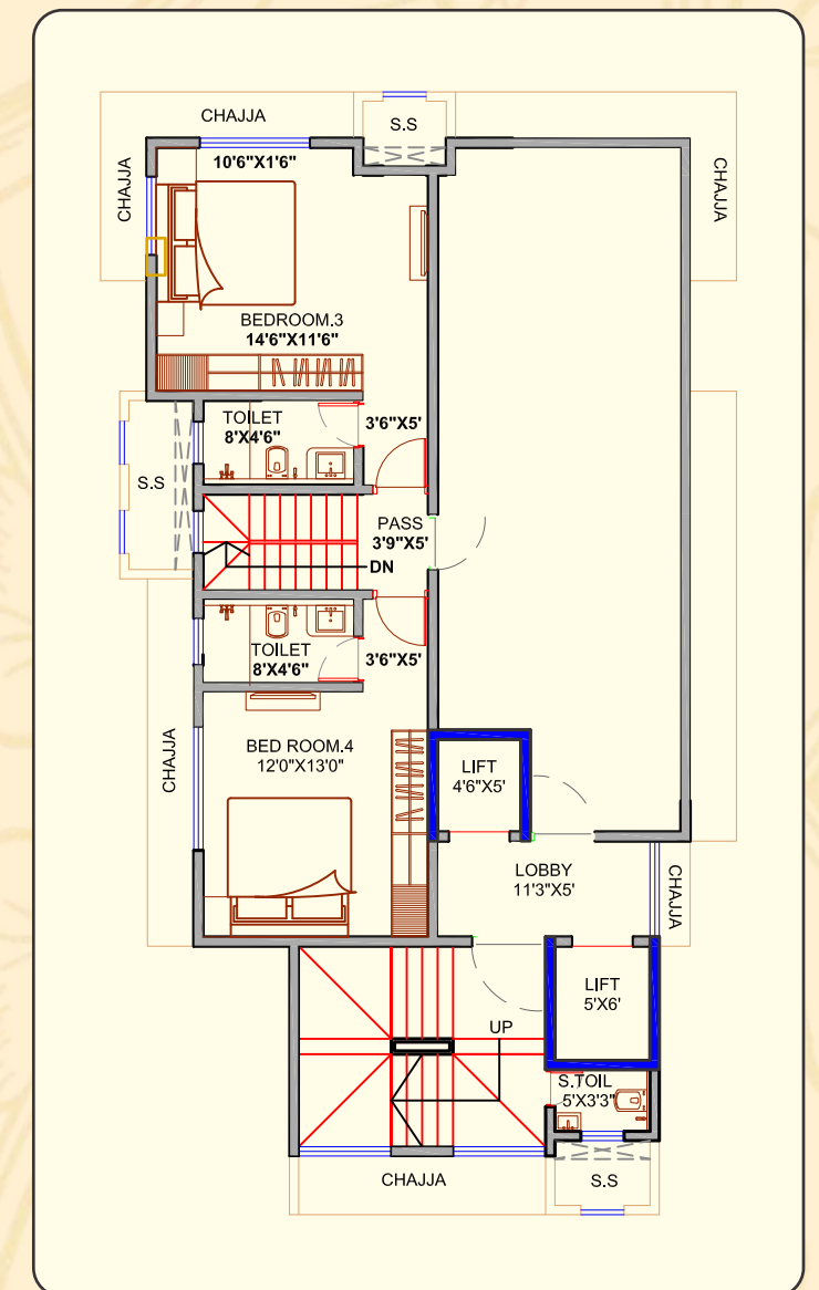
7TH & 14TH, DUPLEX - UPPER LEVEL FLOOR PLAN
