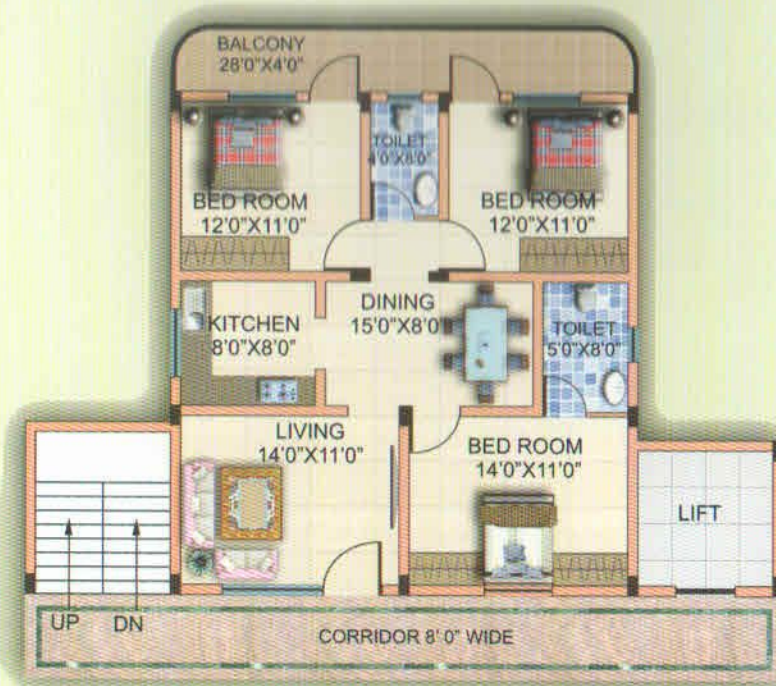
3 BHK Plan -1330sft.
