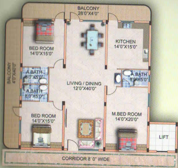
3 BHK Plan -2640sft.
