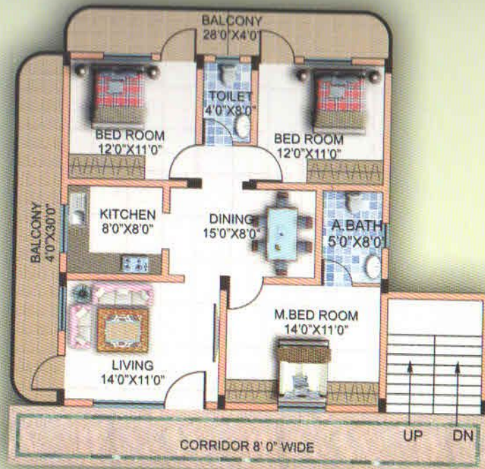
3 BHK Plan -1520sft.
