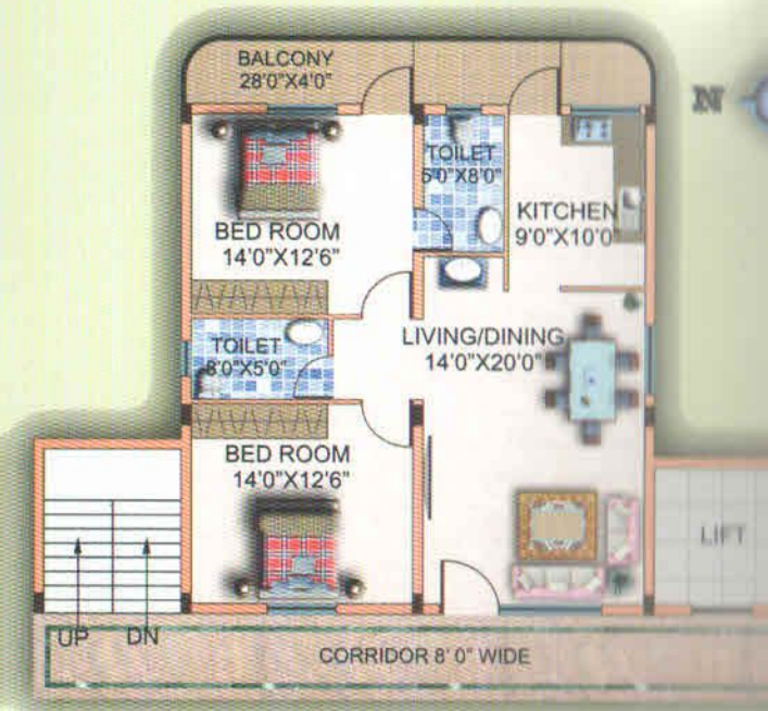
2 BHK Plan -1330sft.
