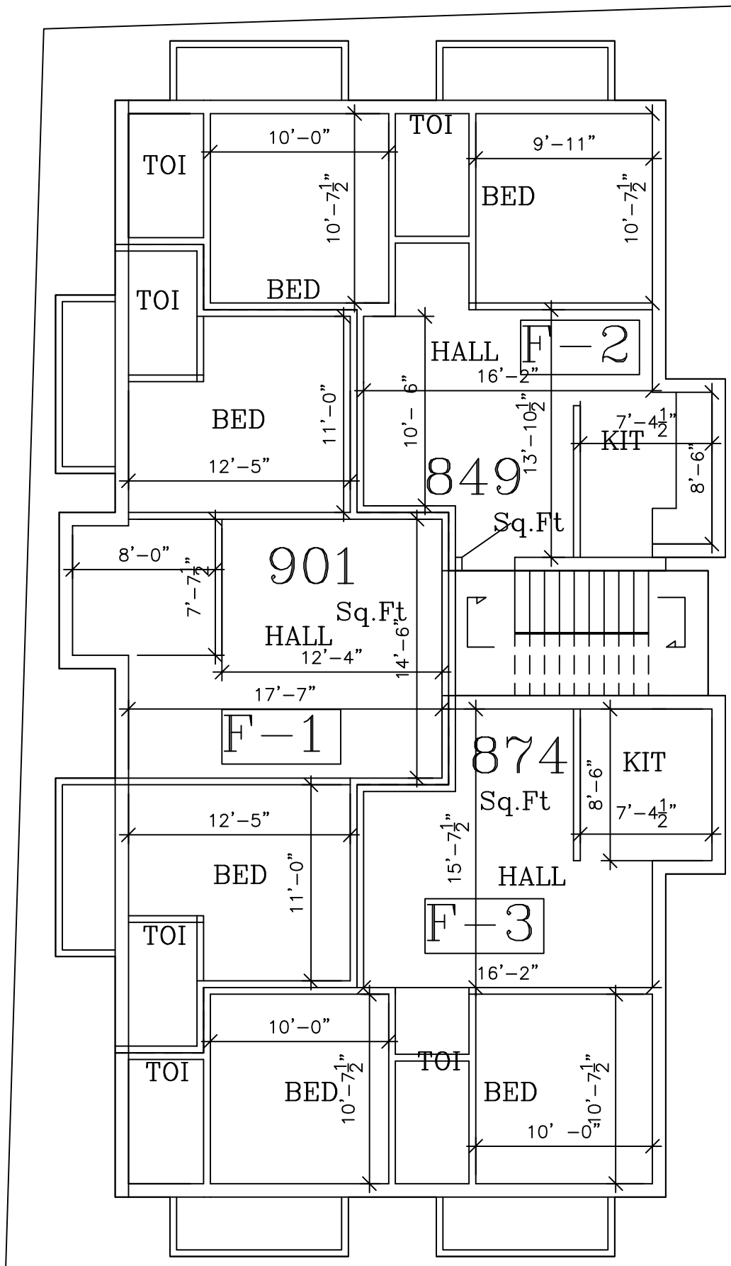
FIRST FLOOR
