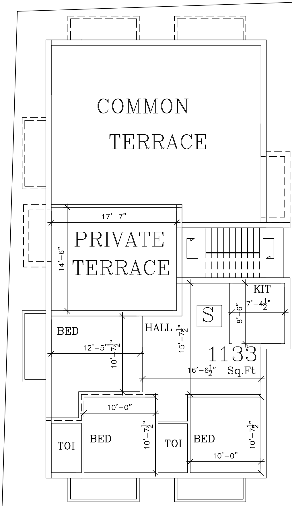
SECOND FLOOR
