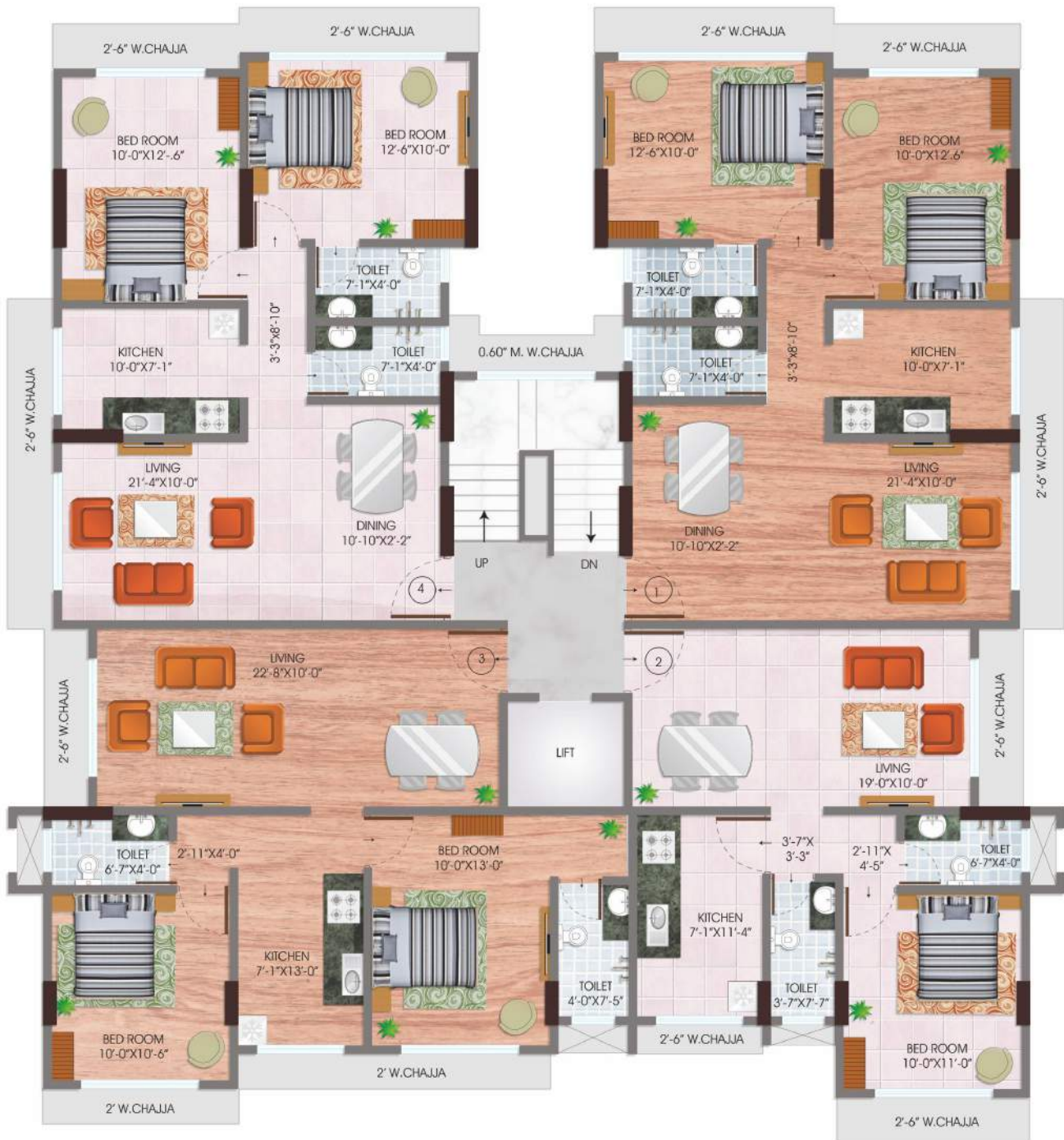
TYPICAL FLOOR PLAN (5TH TO 6TH)
